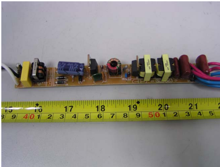
EBA-013L2A-T5: Component View
