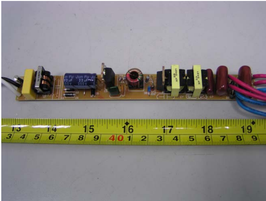
EBA-008L2A-T5: Component View
