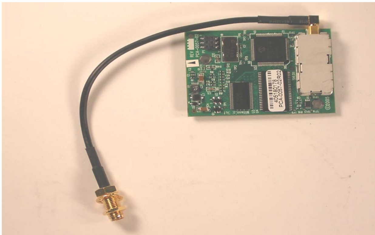
Module top view
