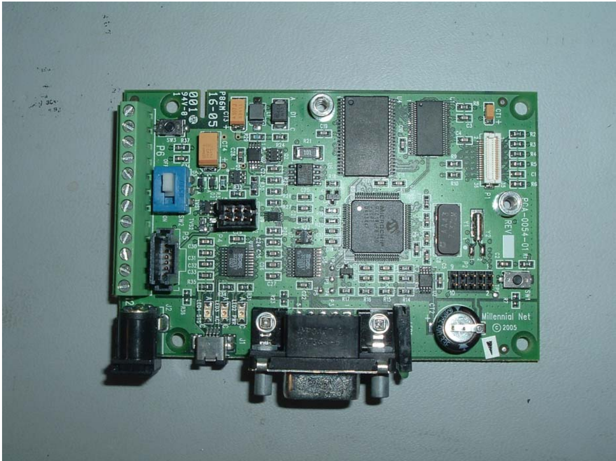
MG-542 Application Board Top Photo
