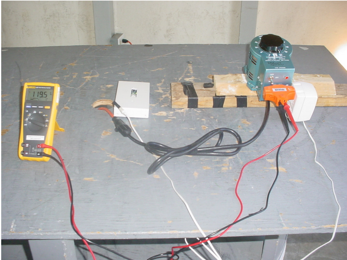
Voltage Variation
