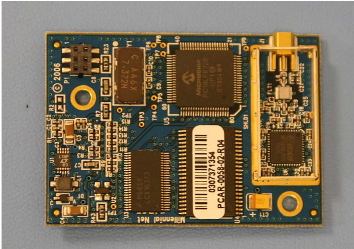
Radio Module Board Top View, No Shield
