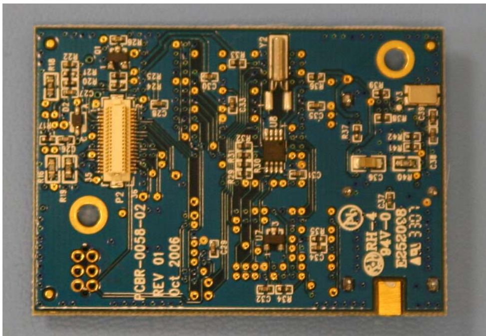
Radio Module Board Bottom View
