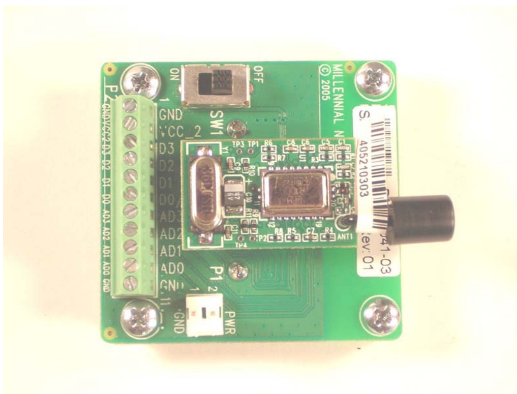
Top view of endnode PCB attached to terminal PCB
