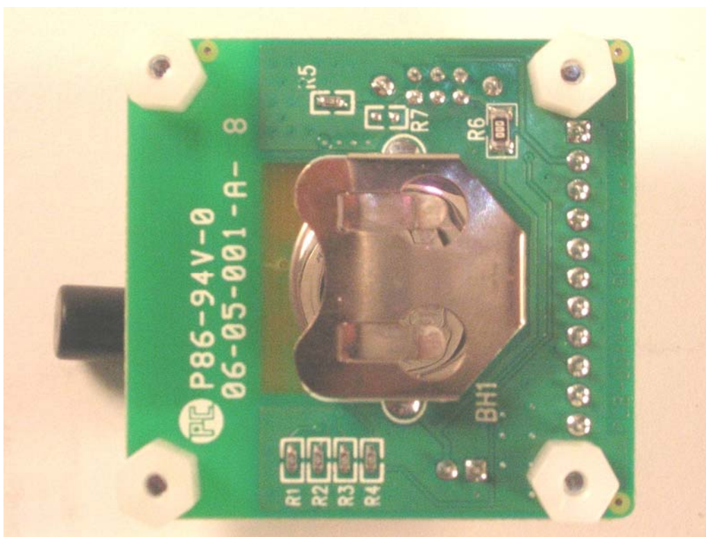
Bottom of terminal PCB
