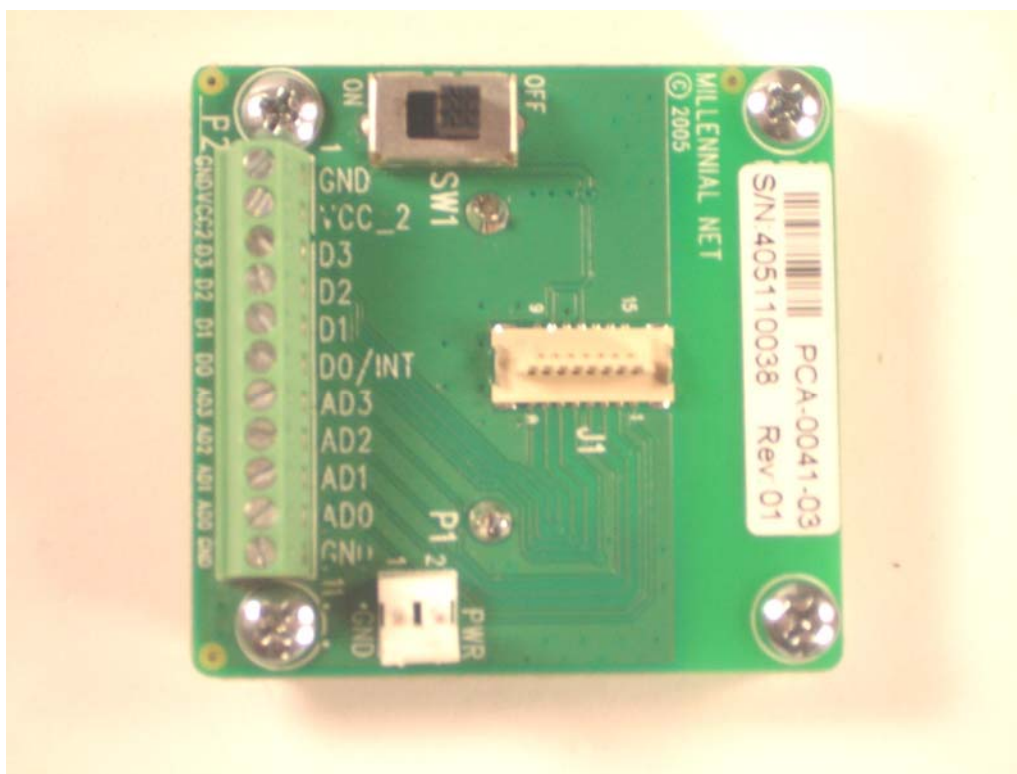
Top view of terminal PCB without endnode PCB
