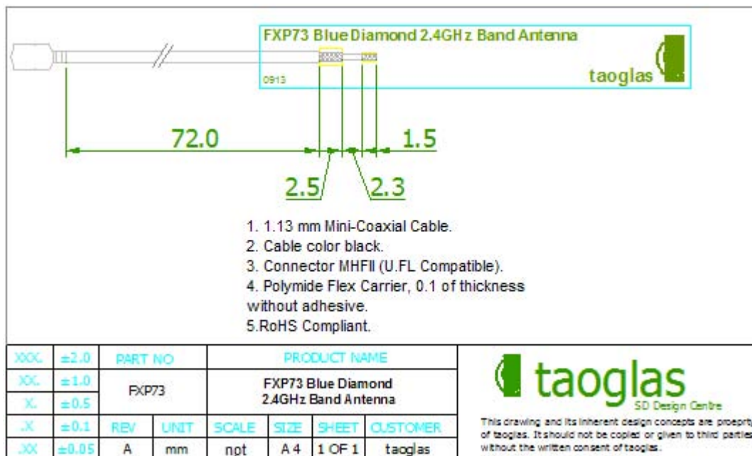
Figure 11. Mechanical Drawing for the FXP73 Antenna.
