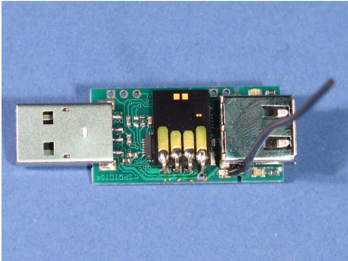
Photograph 1: PCB bottom view
