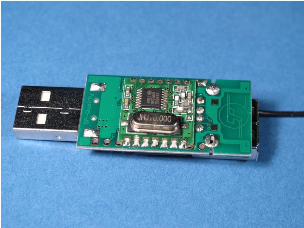
Photograph 2: PCB top view
