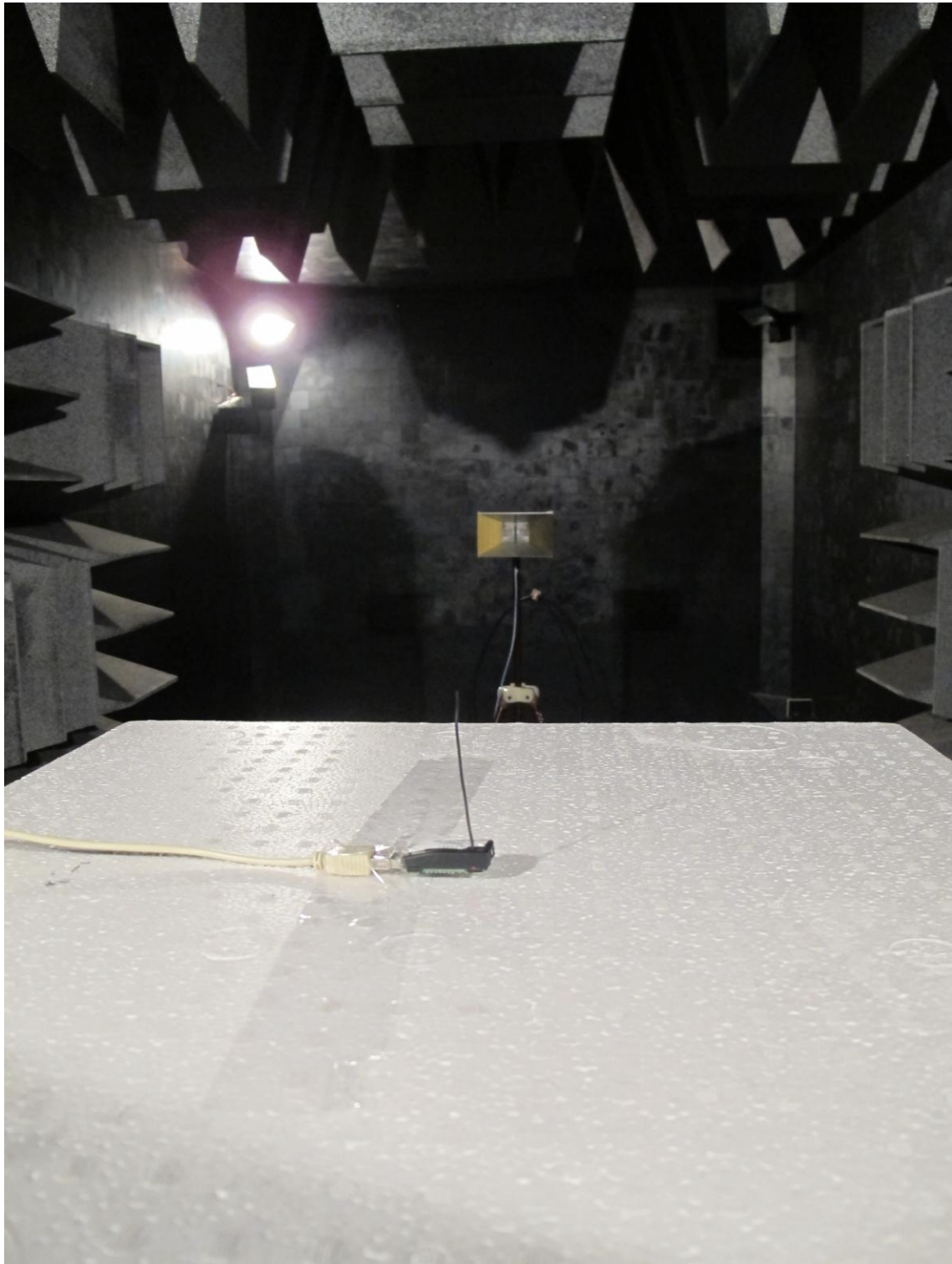
Photograph 4: Radiated emissions test set up > 1000 MHz
