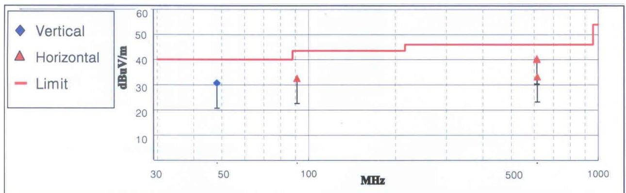
< Fig 6. Radiated emission result >
