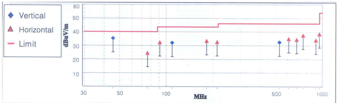
&lt; Fig 5. Radiated emission result _ Digital &gt;
