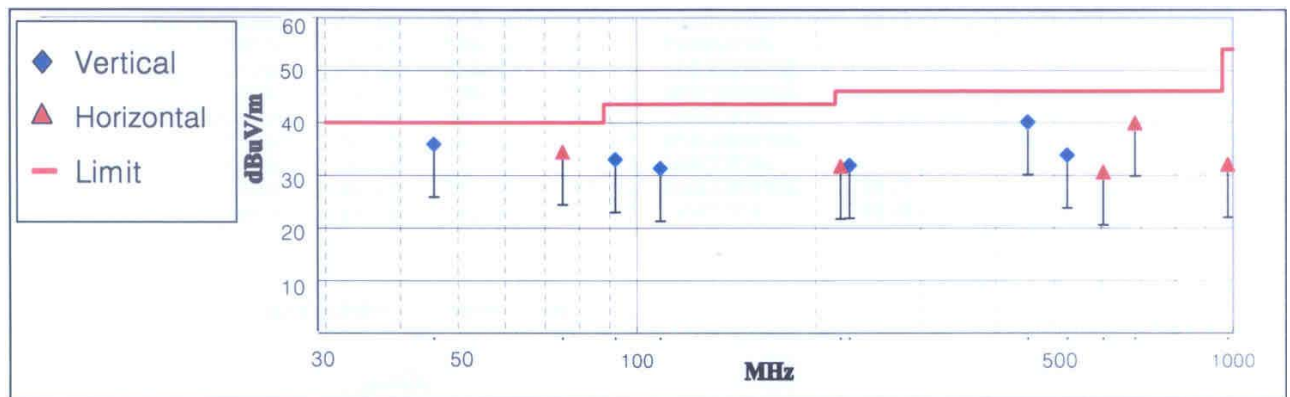
< Fig 4. Radiated emission result _ Analog >
