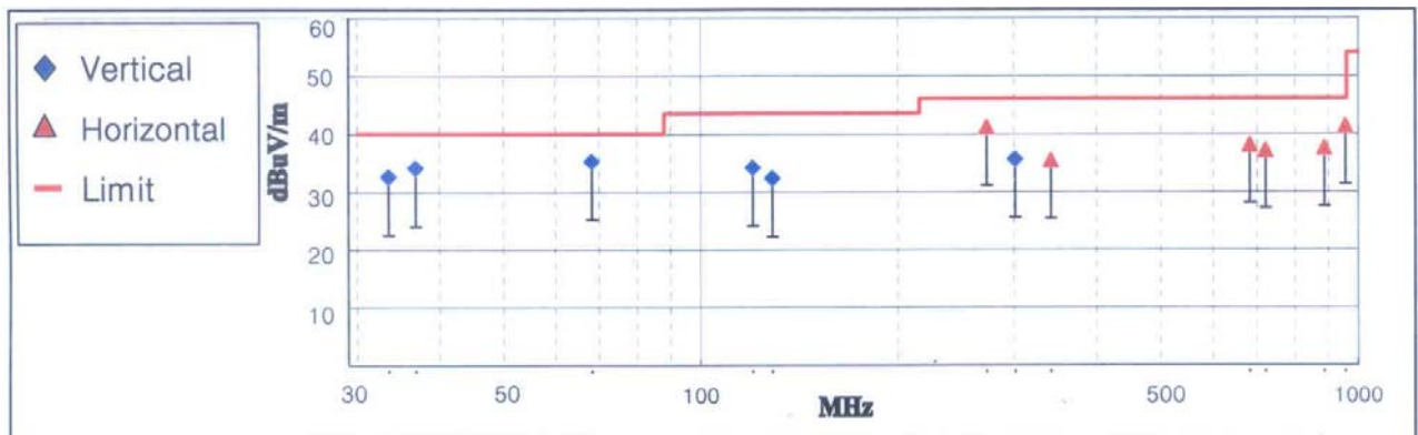
&lt; Fig 5. Radiated emission result _ Digital &gt;
