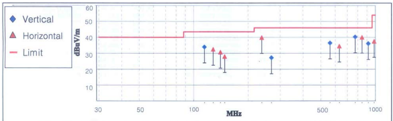
< Fig 6. Radiated emission result >
