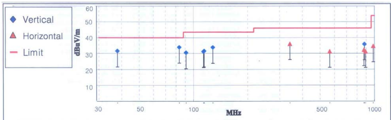
< Fig 4. Radiated emission result _ Analog >
