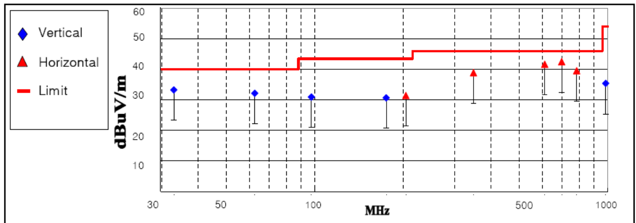
< Fig 6. Radiated emission result _ DVD mode >
