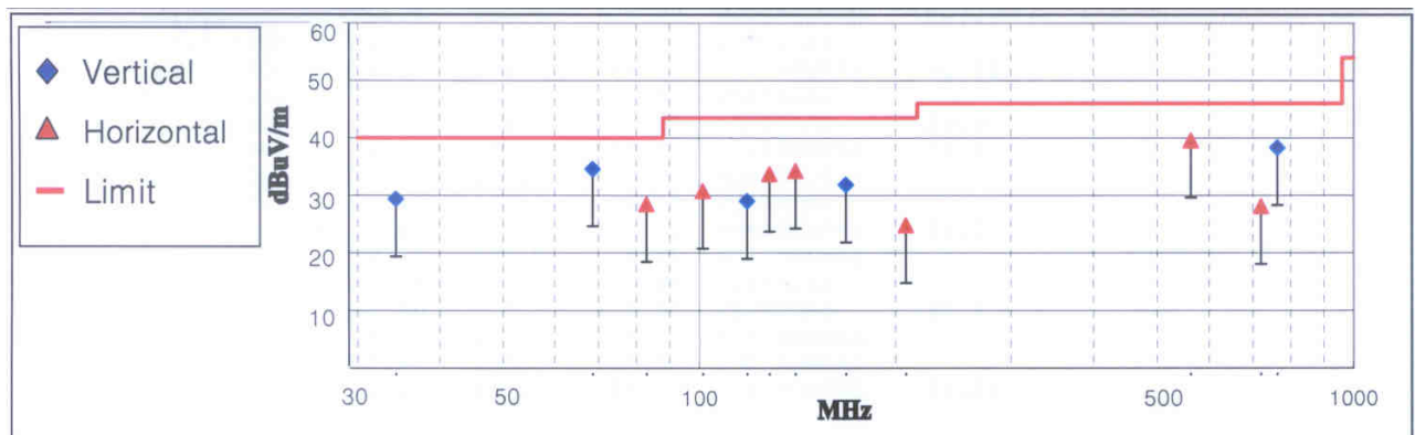
< Fig 4. Radiated emission result _ PC mode >
