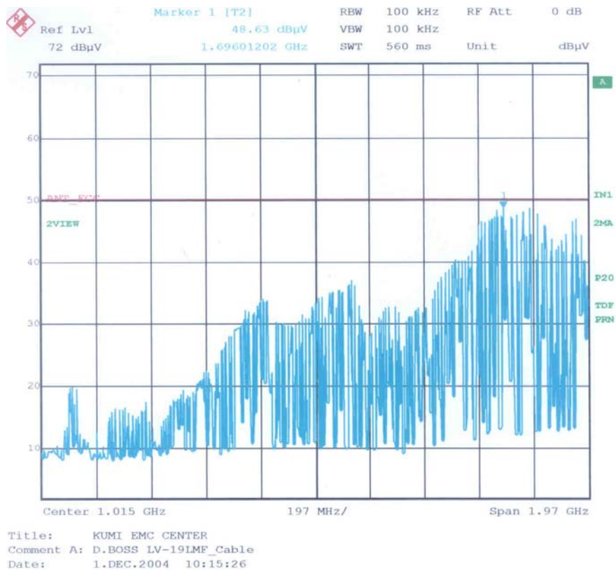
< Fig 7. Antenna power conduction result _ Cable channel >
