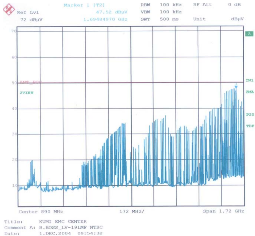
< Fig 6. Antenna power conduction result >
