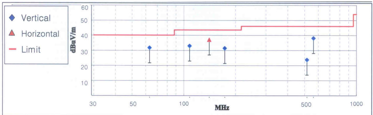
< Fig 5. Radiated emission result _ DVD mode>
