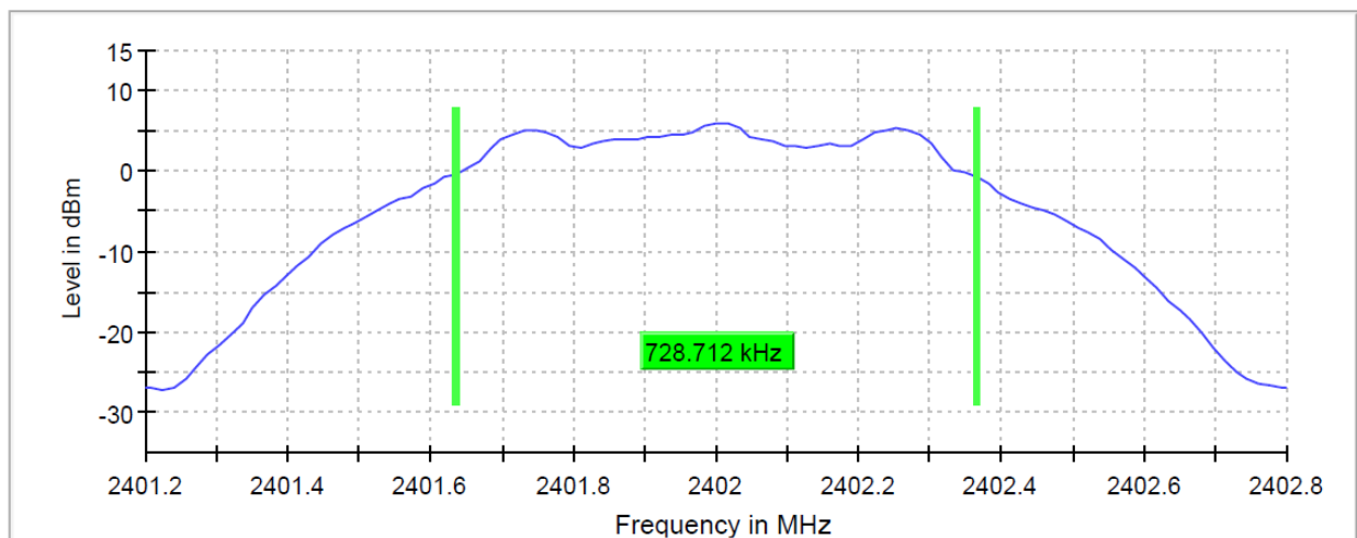
6 dB Bandwidth
