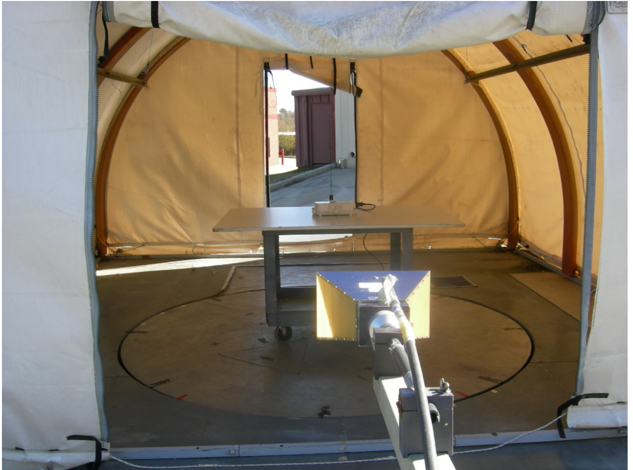
Figure 2: Radiated Emissions
