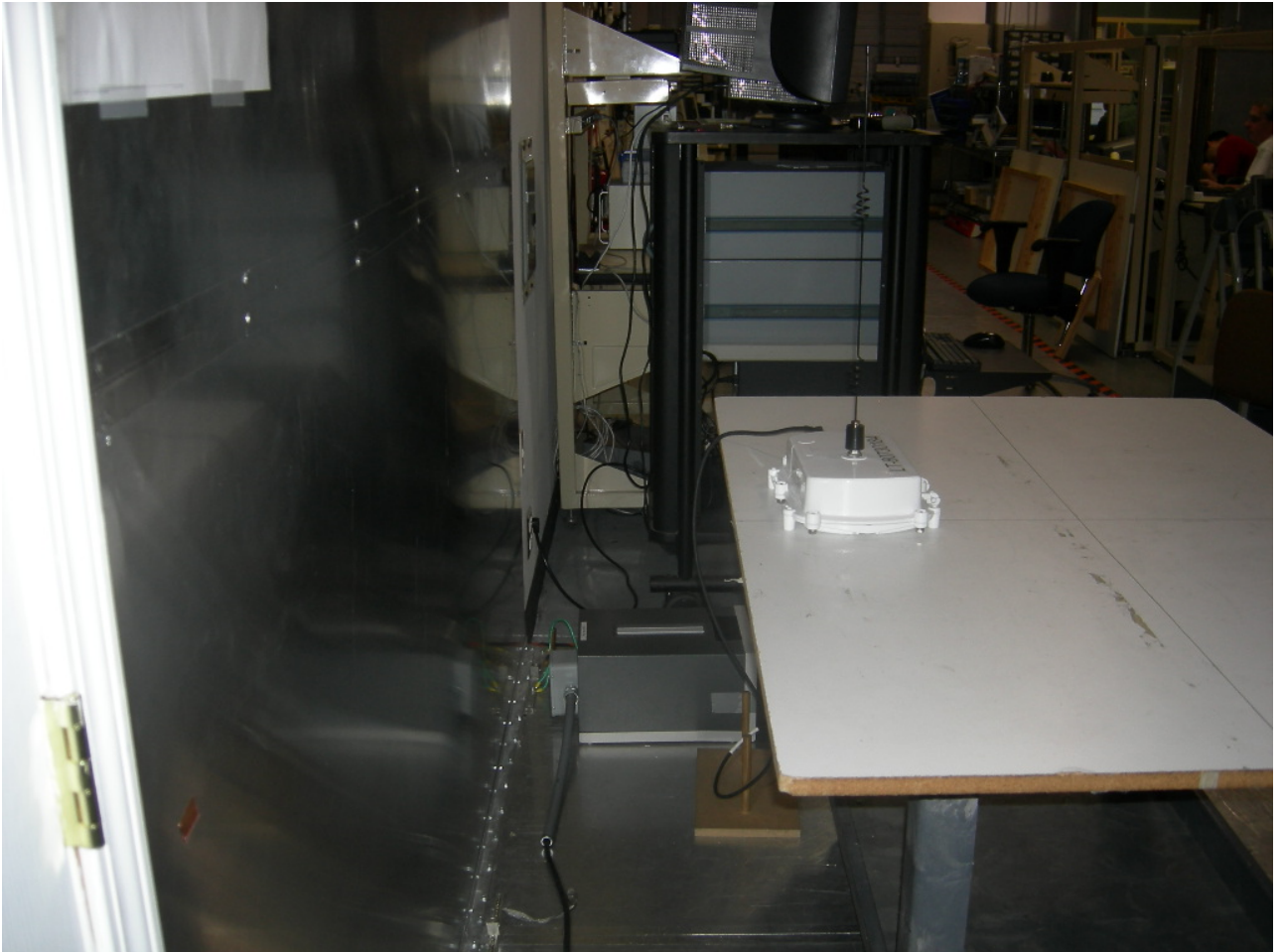
Figure 4: Conducted Emissions
