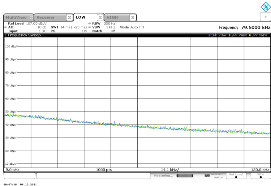
Figure 1: Reference plot for Radiated Spurious Emissions – 9 kHz – 150 kHz – Mode 1
