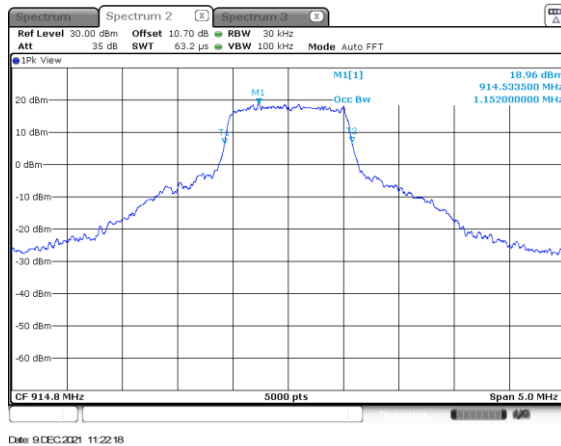
Figure 2.4.6-13: Mode 1 – 99% BW – MCH – MCS0
