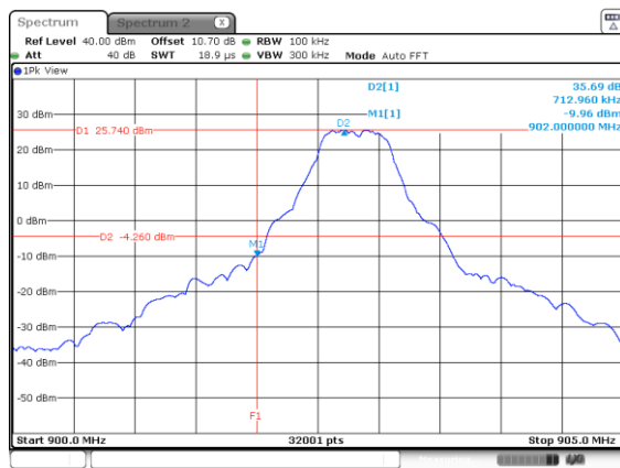
Figure 2.6.6-3: Lower Band edge – Mode 2 – MCS5
