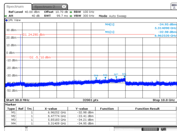
Figure 2.7.6-6:30MHz – 10GHz – MCH – Mode 3
