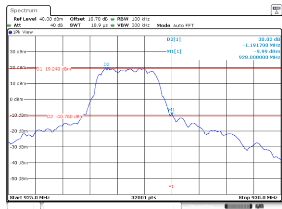
Figure 2.6.6-2: Higher Band edge – Mode 1 – MCS0
