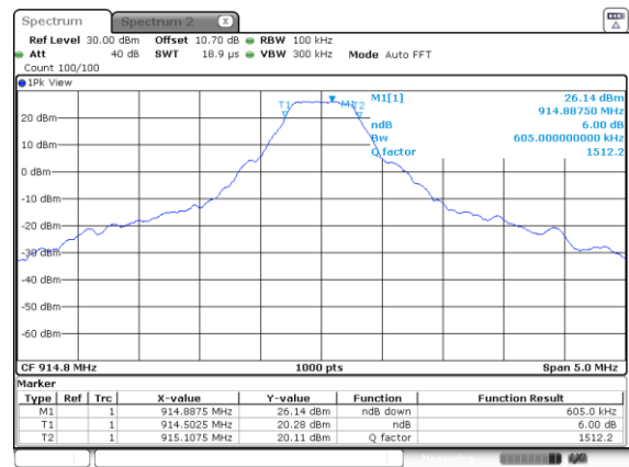
Figure 2.4.6-6: Mode 3 – 6 dB BW – MCH - MCS3
