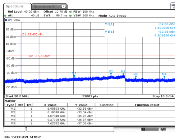
Figure 2.7.6-9:30MHz – 10GHz – HCH – Mode 3
