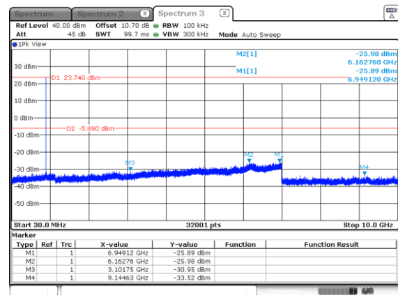
Figure 2.7.6-4:30MHz – 10GHz – MCH – Mode 1
