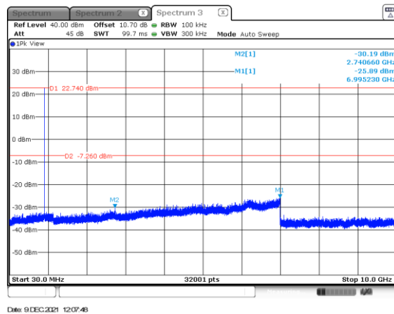
Figure 2.7.6-7:30MHz – 10GHz – HCH – Mode 1
