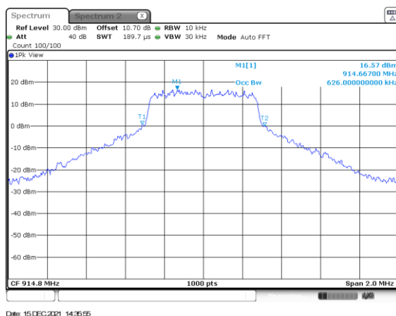
Figure 2.4.6-15: Mode 3 – 99% BW – MCH – MCS3
