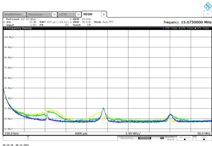
Figure 2: Reference plot for Radiated Spurious Emissions– 150 kHz – 30MHz – Mode 1 Note: Emissions above the noise floor are ambient not associated with the EUT.
