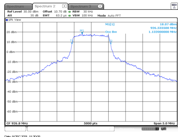
Figure 2.4.6-16: Mode 1 – 99% BW – HCH – MCS0
