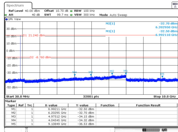
Figure 2.7.6-2:30MHz – 10GHz – LCH – Mode 2
