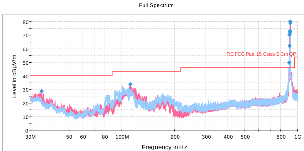
Figure 3: Reference plot for Radiated Spurious Emissions – 30 MHz – 1 GHz – Mode 1 Note: Emissions above the noise floor do not falls within restricted bands.
