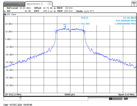
Figure 2.4.6-14: Mode 2 – 99% BW – MCH - MCS5
