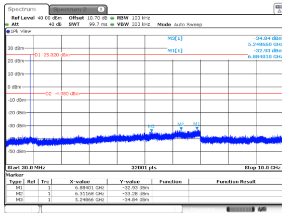
Figure 2.7.6-1:30MHz – 10GHz – LCH – Mode 1
