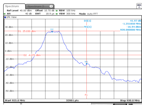
Figure 2.6.6-6: Higher Band edge – Mode 3 – MCS3
