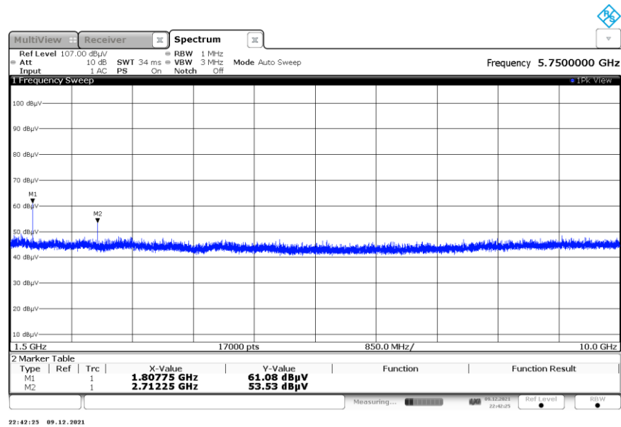
Figure 5: Reference plot for Radiated Spurious Emissions – 1.5 GHz – 10 GHz – Mode 1 Note: Only emissions within restricted bands were evaluated.
