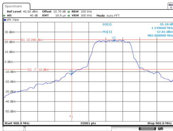
Figure 2.6.6-1: Lower Band edge – Mode 1 – MCS0
