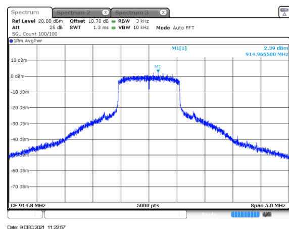
Figure 2.5.6.3-4: Mode 1 – PSD – MCH – MCS0
