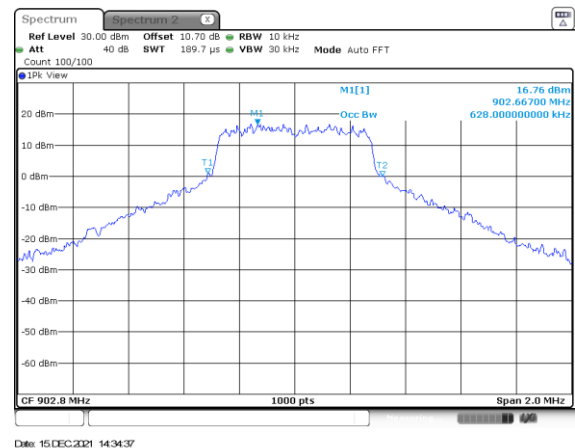
Figure 2.4.6-12: Mode 3 – 99% BW – LCH – MCS3
