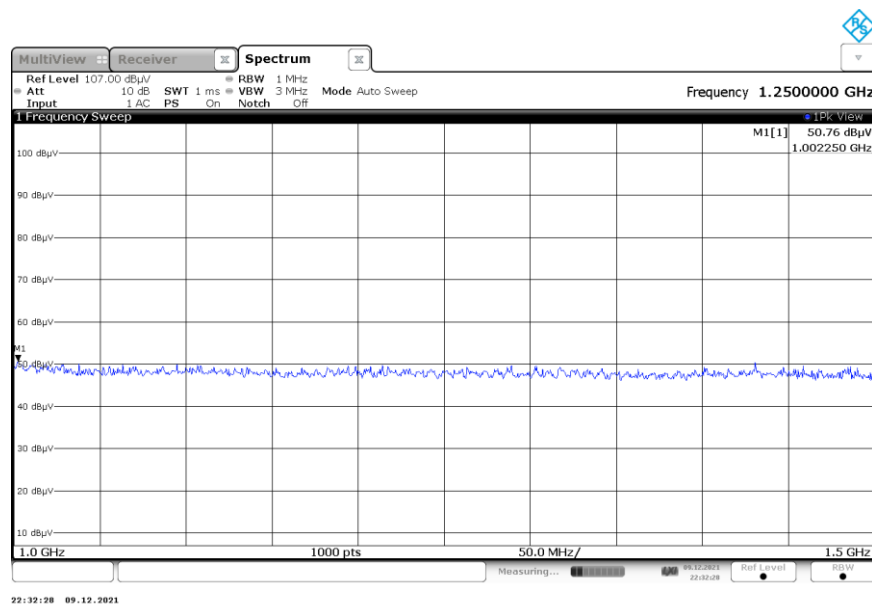
Figure 4: Reference plot for Radiated Spurious Emissions – 1 GHz – 1.5 GHz – Mode 1
