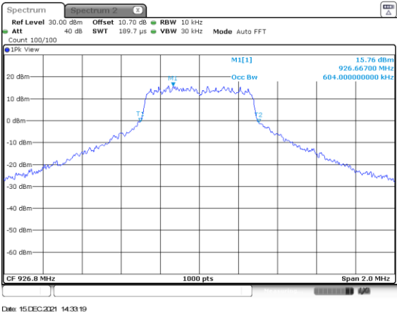
Figure 2.4.6-18: Mode 3 – 99% BW – HCH – MCS3
