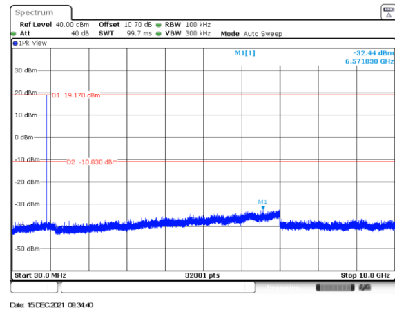
Figure 2.7.6-8:30MHz – 10GHz – HCH – Mode 2
