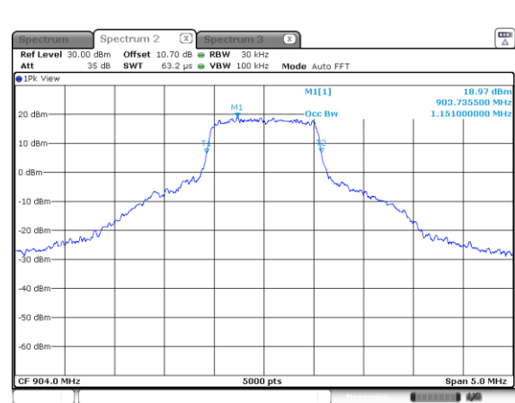
Figure 2.4.6-10: Mode 1 – 99% BW – LCH MCS0
