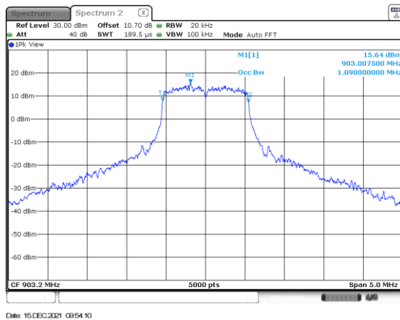
Figure 2.4.6-11: Mode 2 – 99% BW – LCH – MCS5
