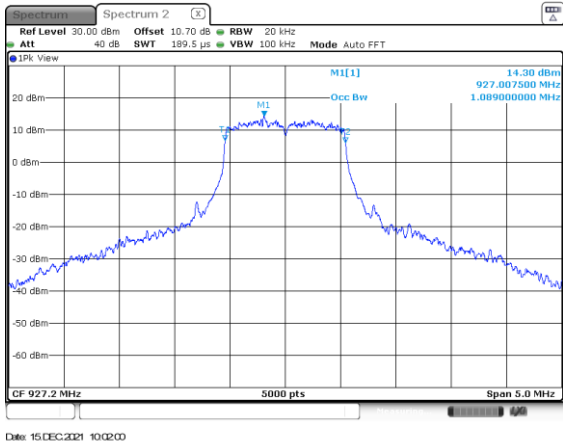
Figure 2.4.6-17: Mode 2 – 99% BW – HCH – MCS5
