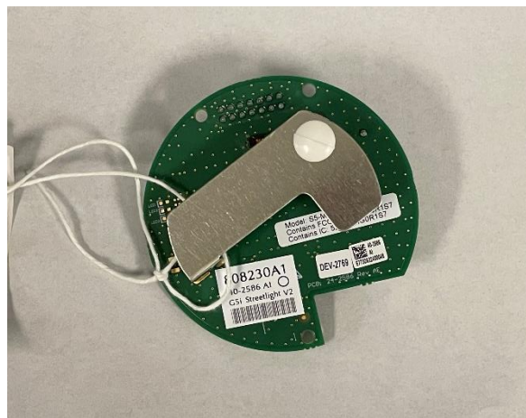
Figure 1.4.1-2: Rear End of the Radiated EUT Module
