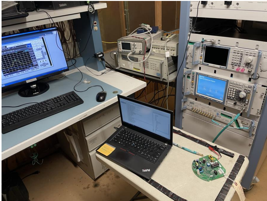
Figure:7 – Test Set up – Antenna Port measurements
