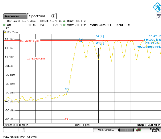
Figure 2.10.6-1: Lower Band edge – Mode 1 – 200kbps
