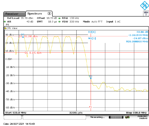
Figure 2.10.6-2: Higher Band edge – Mode 1 – 200kbps
