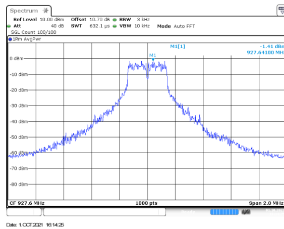
Figure 2.9.6-3: Mode 5 – PSD – HCH – MCS2
