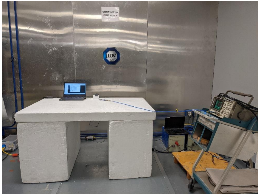
Figure 5 – Test Set up – Conducted Emissions
