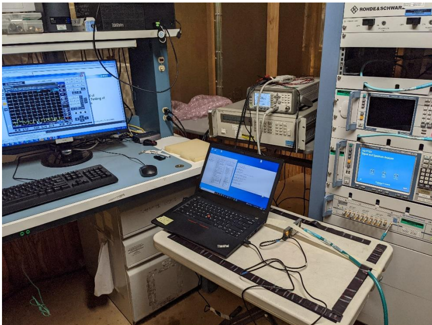
Figure 4 – Test Set up – Antenna Port measurements
