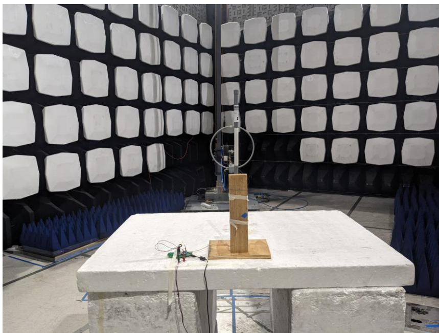
Figure2 – Rear View Test Set up - Radiated Emissions <30 MHz
