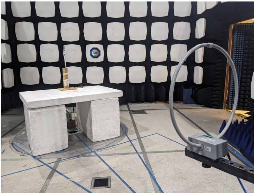
Figure1 – Front View Test Set up - Radiated Emissions <30 MHz
