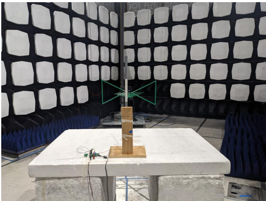
Figure4 – Rear View Test Set up - Radiated Emissions <1 GHz
