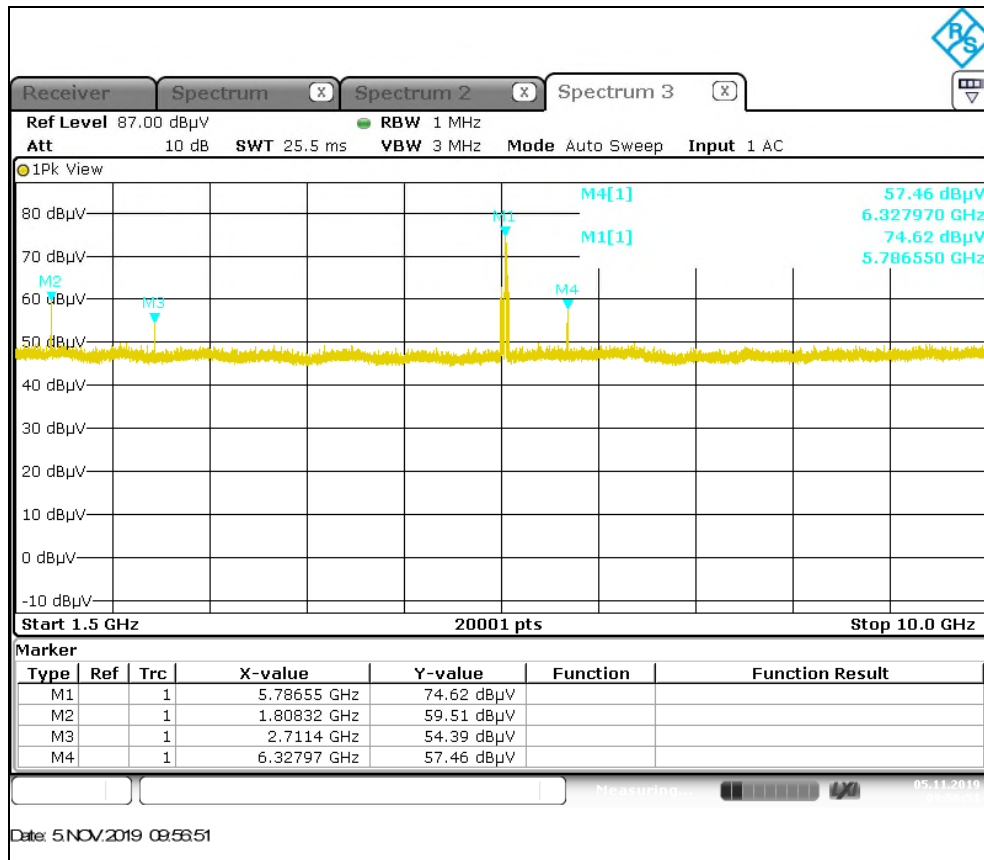
Figure A-4: Radiated Emissions – 1.5GHz-10GHz
