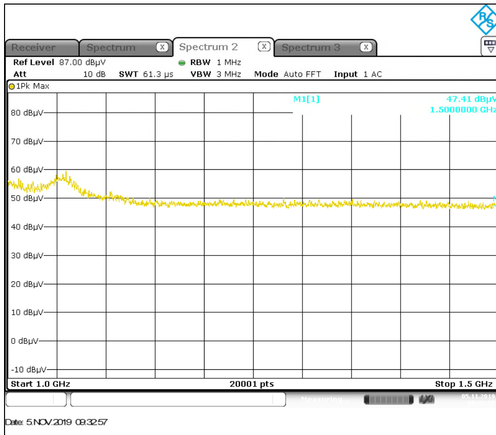
Figure A-4: Radiated Emissions – 1GHz-1.5GHz
