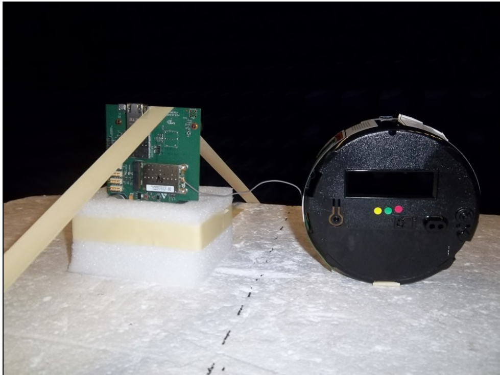
Figure 2: Equipment Under Test – Radiated Emissions Z-orientation
