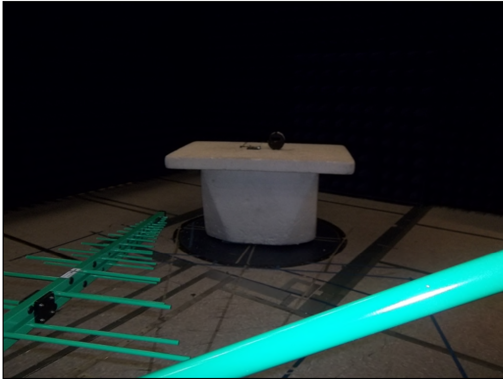
Figure 5: Equipment Under Test – Radiated Emissions <1GHz
