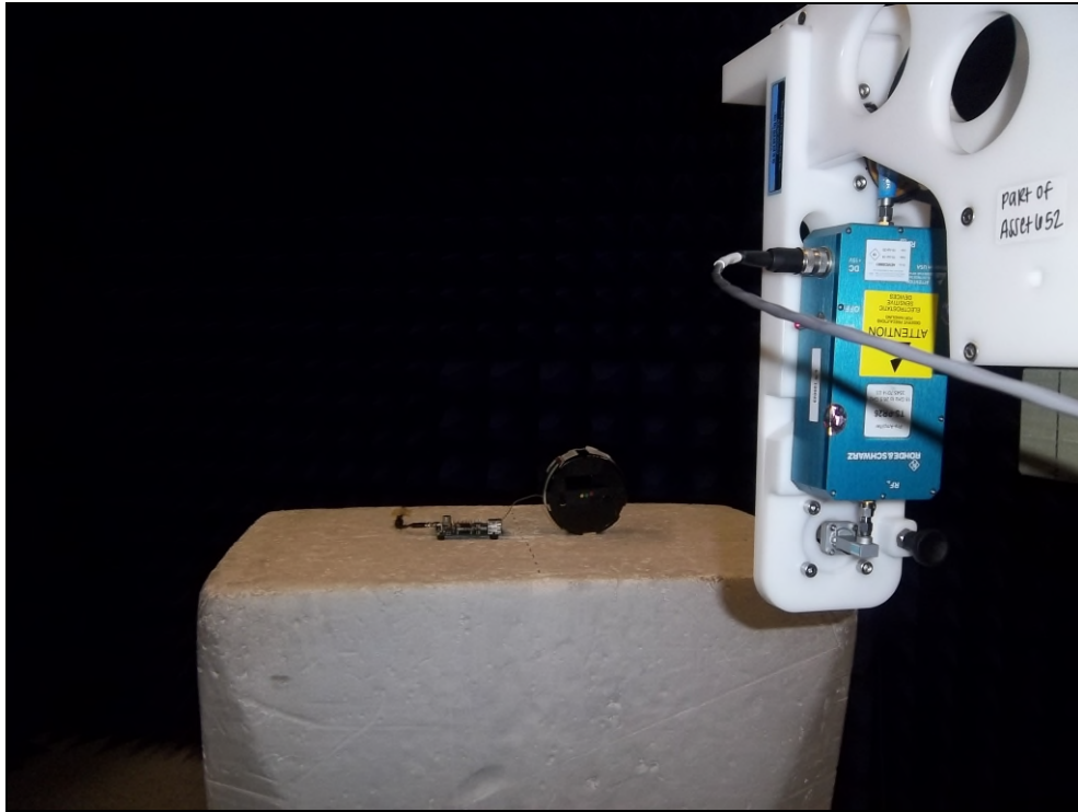
Figure 9: Equipment Under Test – Radiated Emissions >18GHz
