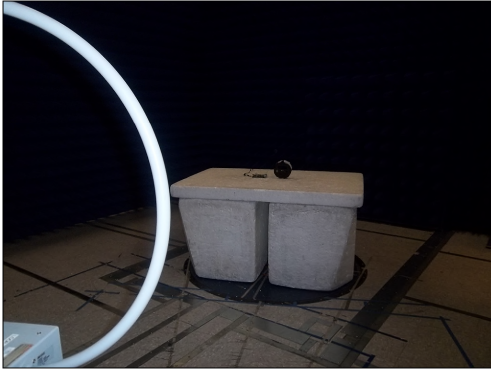
Figure 3: Equipment Under Test – Radiated Emissions <30MHz
