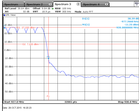
Figure 7.5.1.2-19: Upper Band-edge – Mode 4
