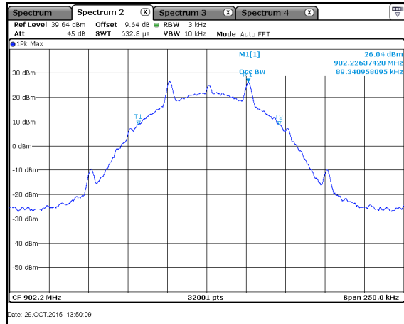
Figure 7.4.4.2-28: 99% BW Low Channel - 50.0kbps
