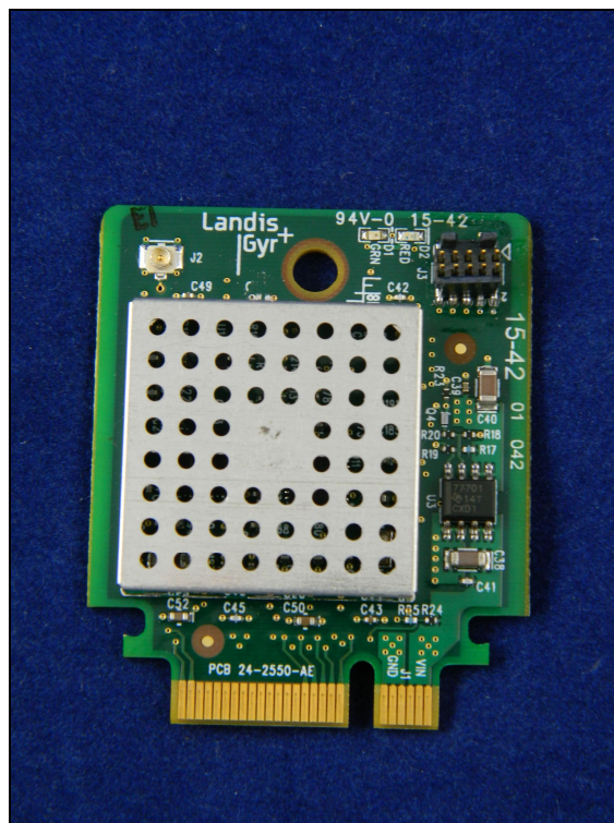
Figure 1: External Photo
