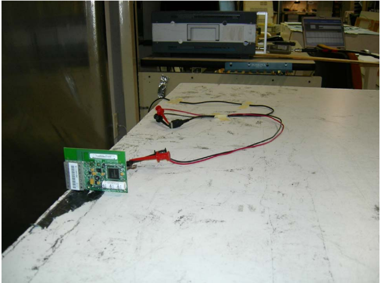
Figure 5: Conducted Emissions
