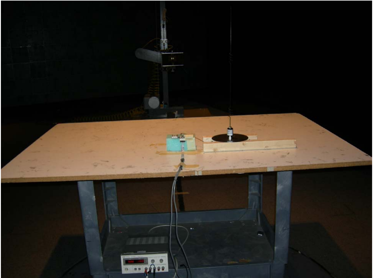
Figure 2: Radiated Emissions – External Antenna
