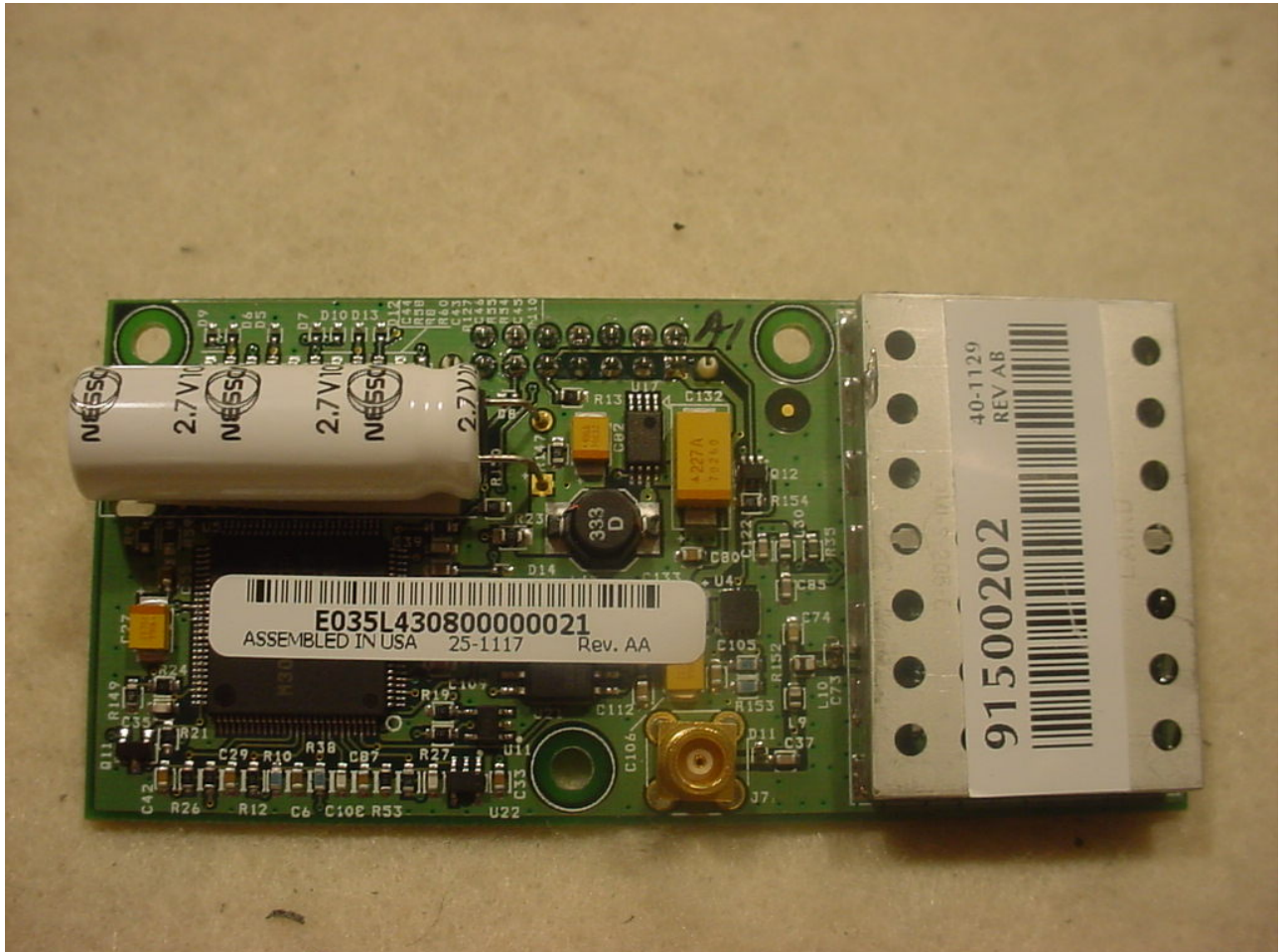
Figure 1: External Antenna PCB with Shields - Front
