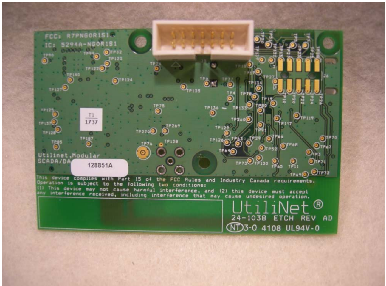
Figure 6: Internal Antenna PCB - Back
