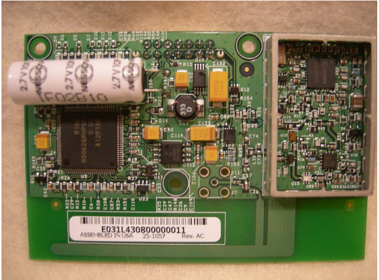
Figure 5: Internal Antenna PCB without Shield – Front
