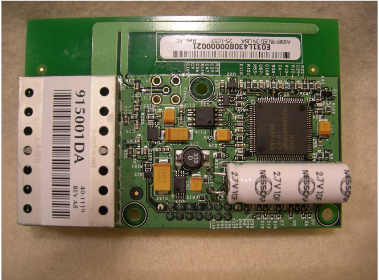
Figure 4: Internal Antenna PCB with Shields – Front
