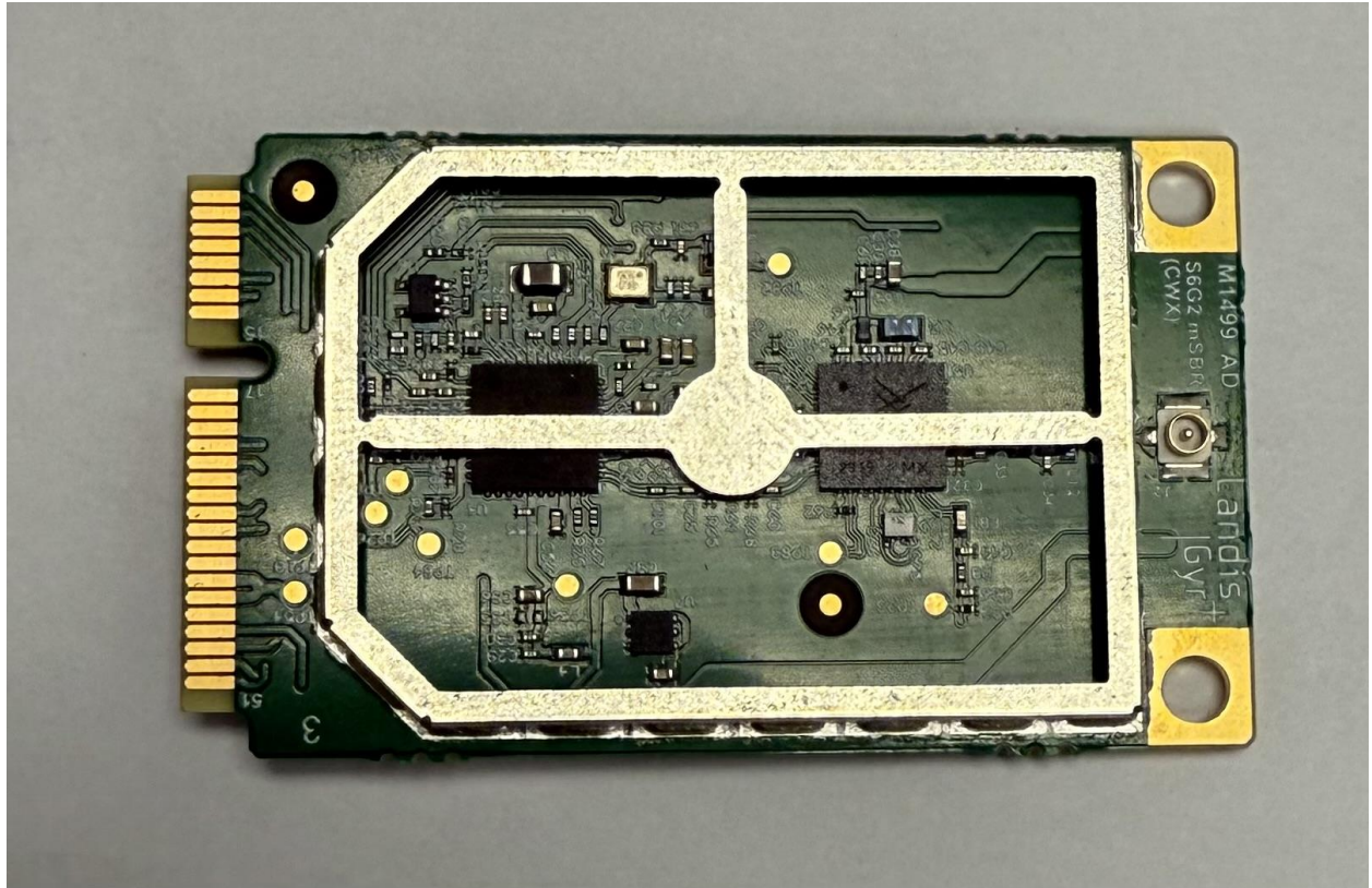
Figure 1: PCB Front without Shields
