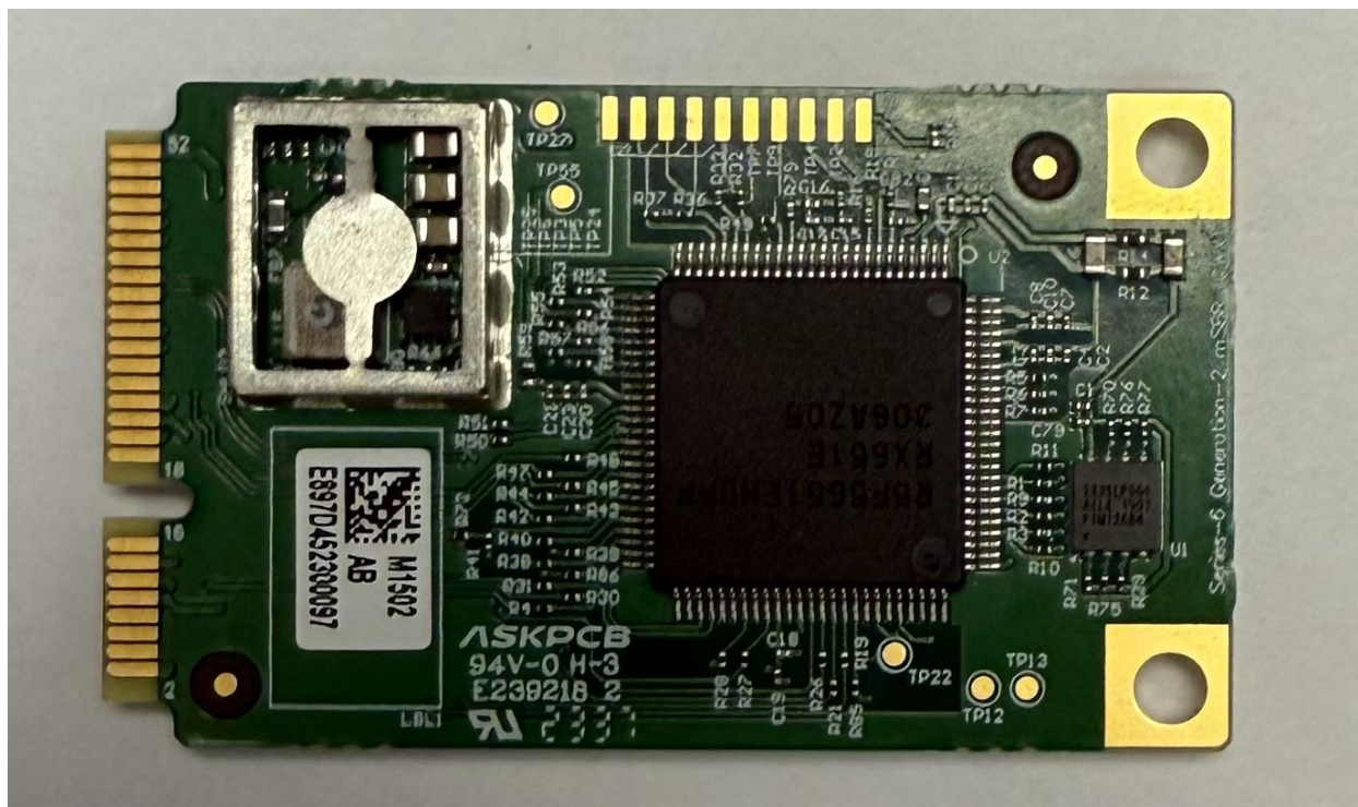
Figure 2: PCB Back without Shields
