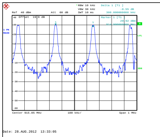
Figure 7.4.1.2-1: Mode 1
