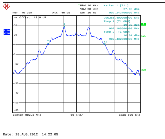
Figure 7.4.4.2-19: 99% BW Low Channel - 115.2kbps
