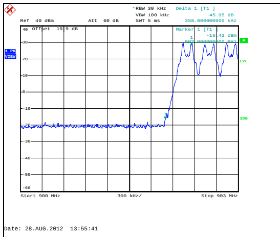
Figure 7.5.1.2-7: Lower Band-edge – Mode 1
