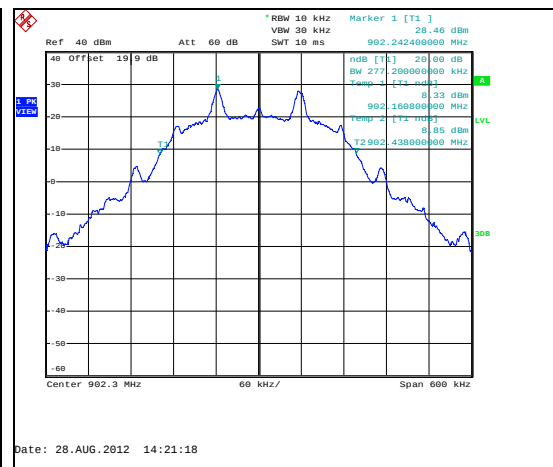
Figure 7.4.4.2-4: 20dB BW Low Channel - 115.2kbps
