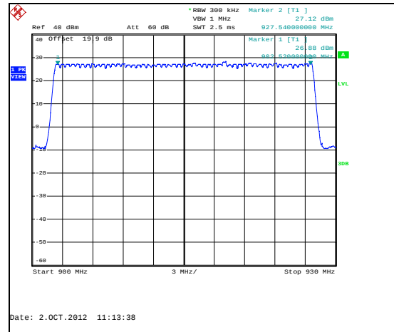
Figure 7.4.2-8: Mode 3 (51 Channels)
