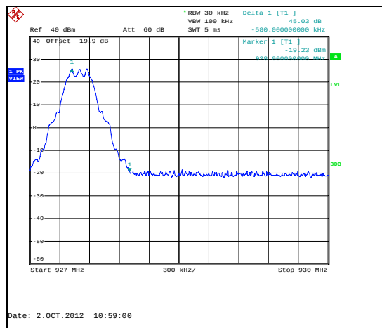
Figure 7.5.1.2-6: Upper Band-edge – Mode 3
