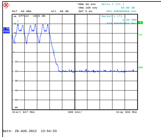
Figure 7.5.1.2-10: Upper Band-edge – Mode 1
