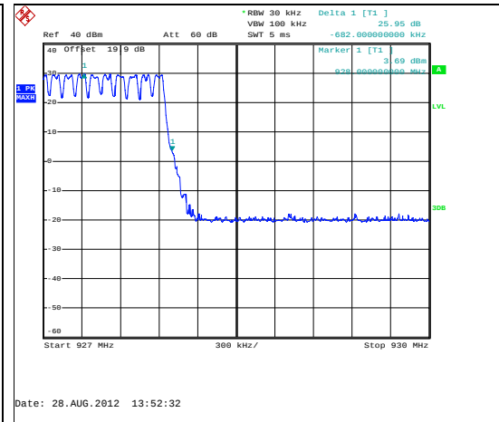
Figure 7.5.1.2-11: Upper Band-edge – Mode 2
