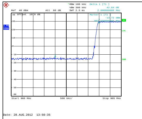
Figure 7.5.1.2-8: Lower Band-edge – Mode 2
