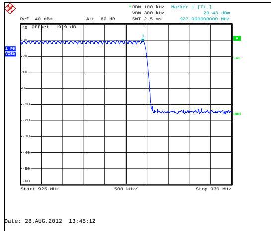
Figure 7.4.2-7: Mode 2 (240 Channels)
