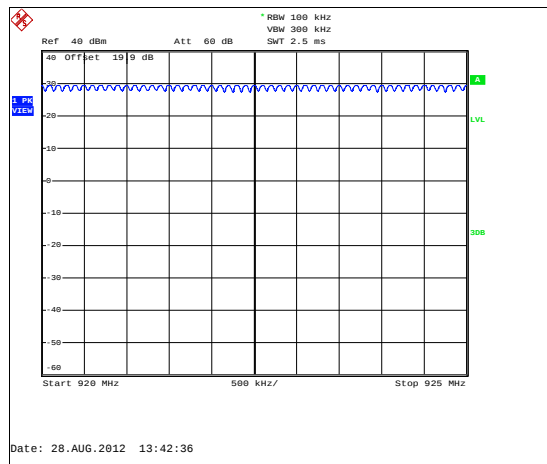
Figure 7.4.2-6: Mode 2 (240 Channels)
