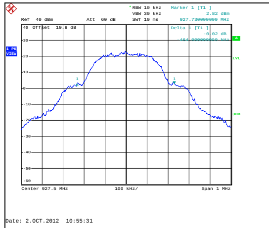
Figure 7.4.4.2-15: 20dB BW High Channel - 300.0kbps
