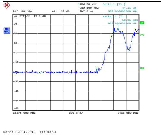
Figure 7.5.1.2-9: Lower Band-edge – Mode 3
