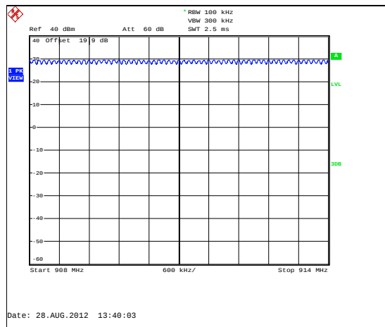
Figure 7.4.2-4: Mode 2 (240 Channels)
