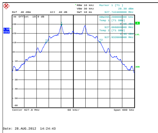
Figure 7.4.4.2-29: 99% BW High Channel - 115.2kbps
