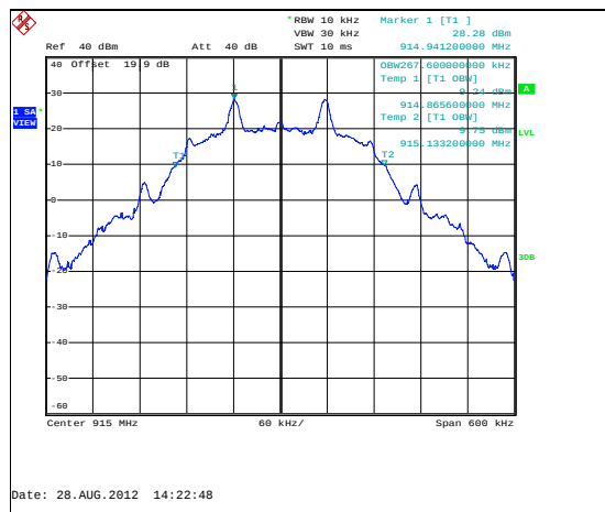
Figure 7.4.4.2-24: 99% BW Mid Channel - 115.2kbps
