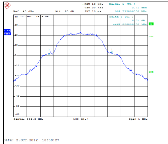
Figure 7.4.4.2-5: 20dB BW Low Channel - 300.0kbps
