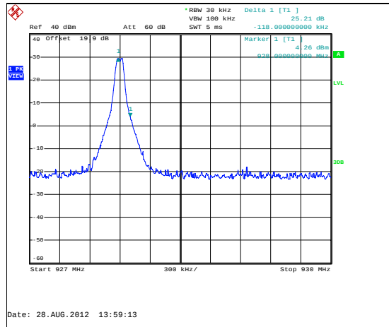
Figure 7.5.1.2-5: Upper Band-edge – Mode 2
