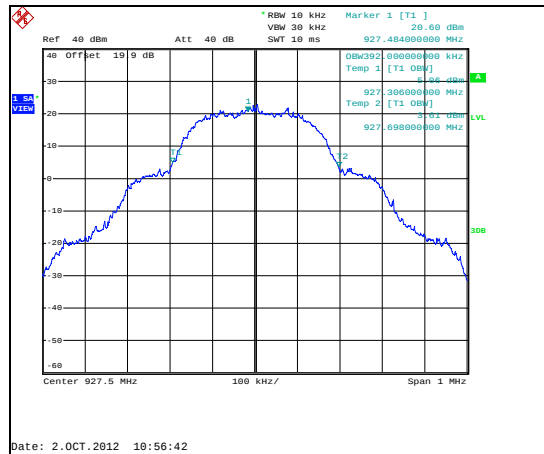
Figure 7.4.4.2-30: 99% BW High Channel - 300.0kbps
