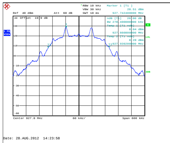
Figure 7.4.4.2-14: 20dB BW High Channel - 115.2kbps
