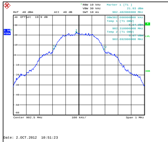
Figure 7.4.4.2-20: 99% BW Low Channel - 300.0kbps
