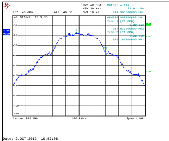
Figure 7.4.4.2-25: 99% BW Mid Channel - 300.0kbps
