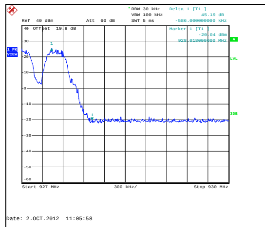
Figure 7.5.1.2-12: Upper Band-edge – Mode 3
