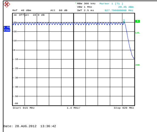
Figure 7.4.2-2: Mode 1 (86 Channels)
