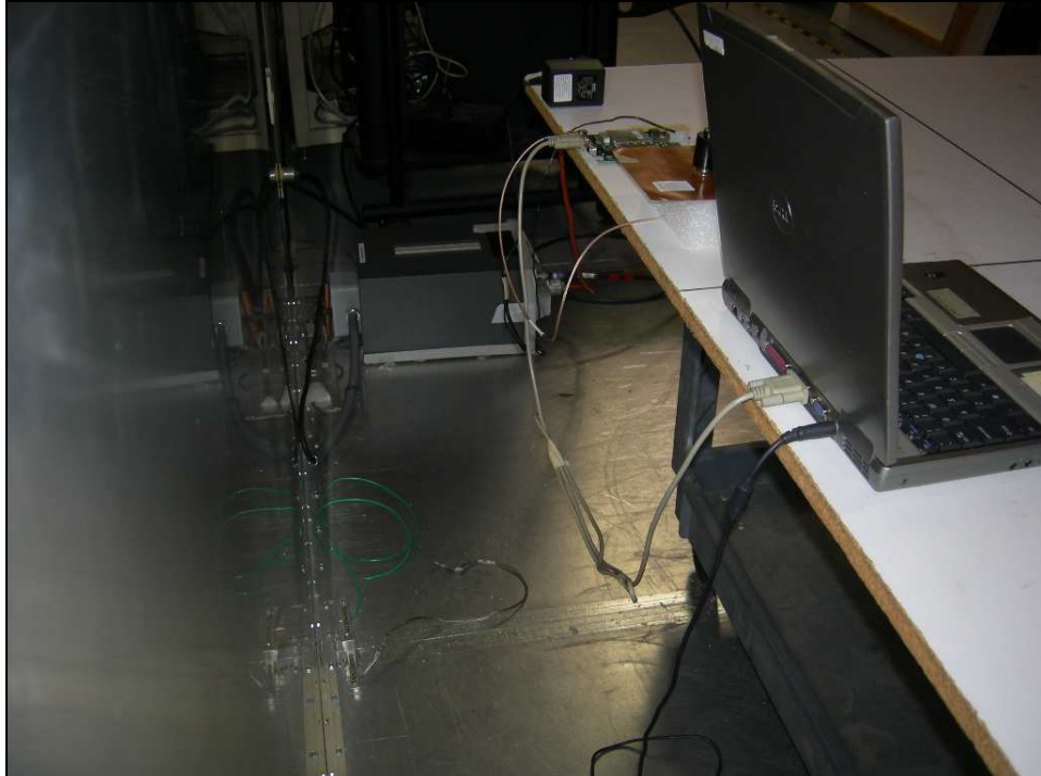
Figure 8: Conducted Emissions
