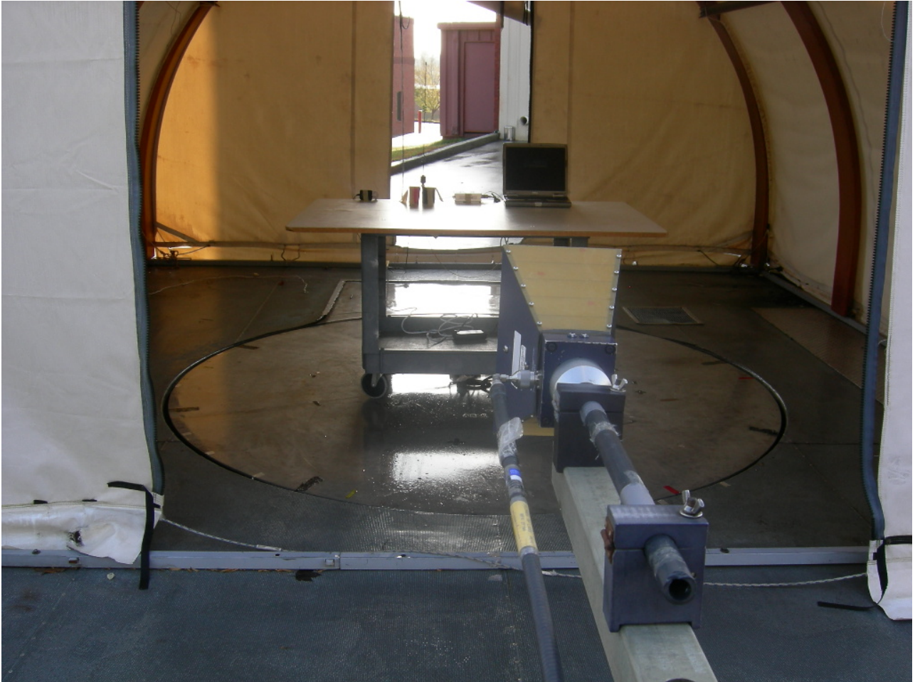
Figure 1: Radiated Emissions
