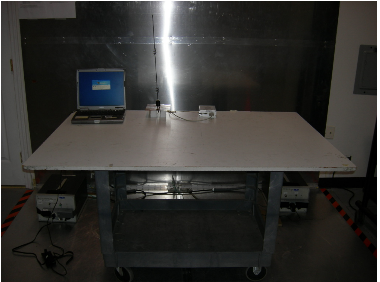
Figure 4: Conducted Emissions
