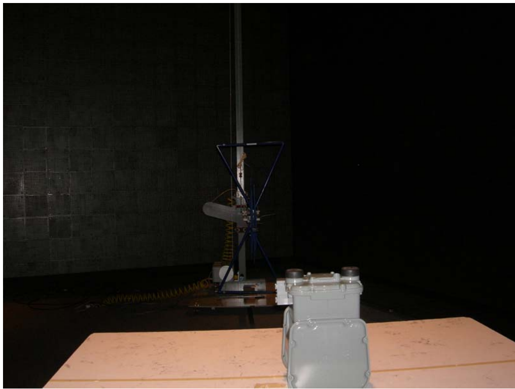
Figure 4: Radiated Emissions
