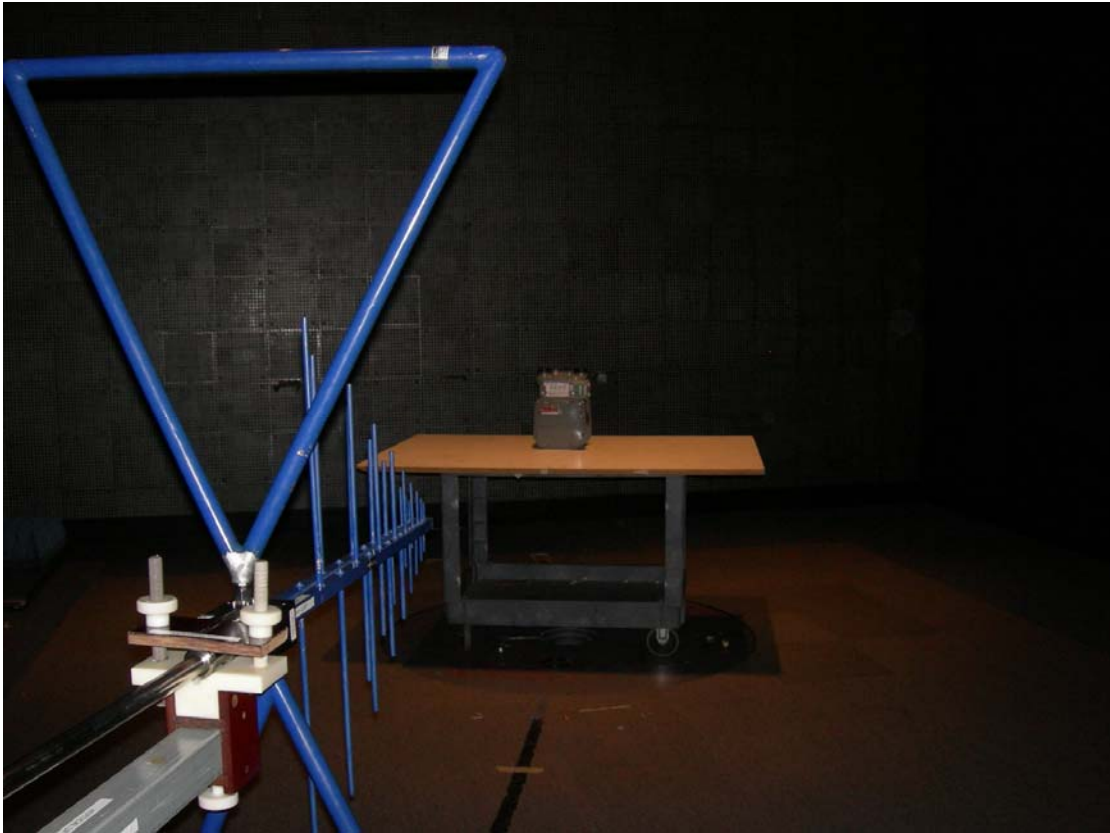
Figure 3: Radiated Emissions
