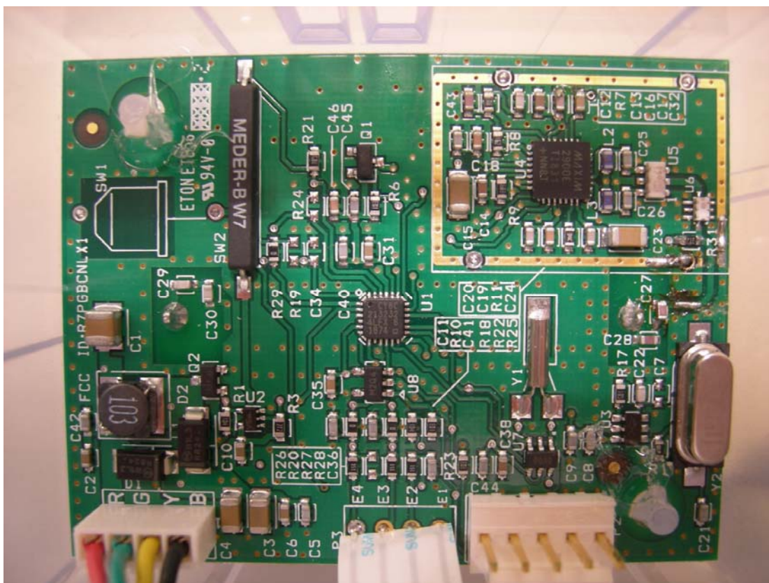
Figure 1: PCB – Front
