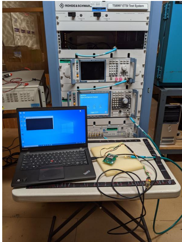
Figure 1: Equipment Under Test – Antenna Port Measurements
