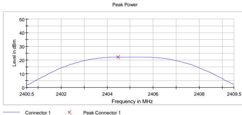
Figure 7.4.2-1: Sample Plot
