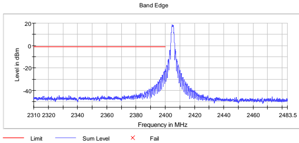
Figure 7.5.1.2-4: Lower Band-edge – Channel 11
