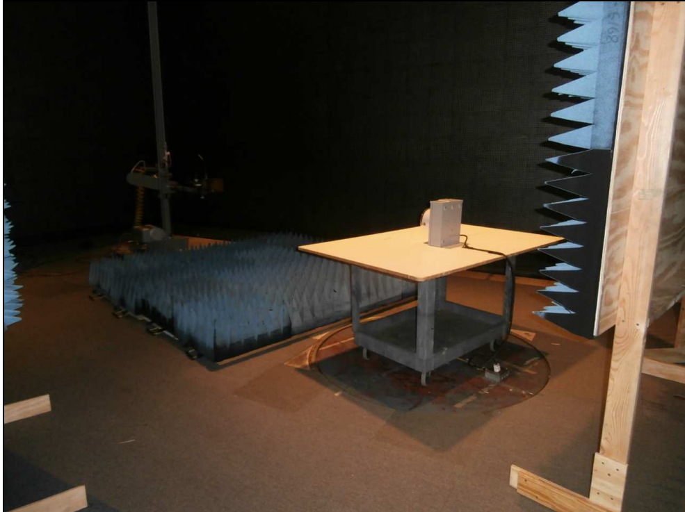
Figure 2: Radiated Emissions
