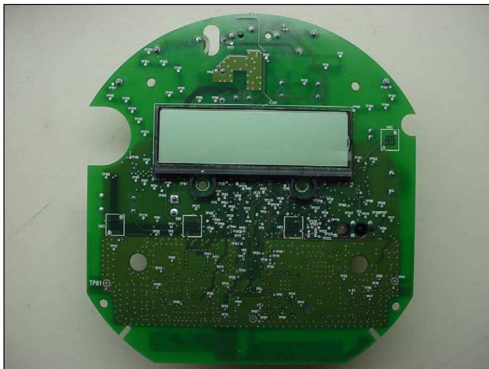
Figure 4: PCB – Back with Display
