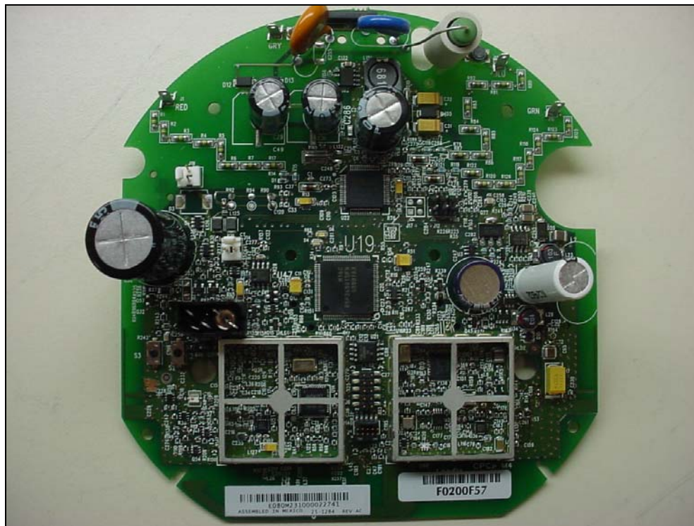
Figure 3: PCB without Shields – Front
