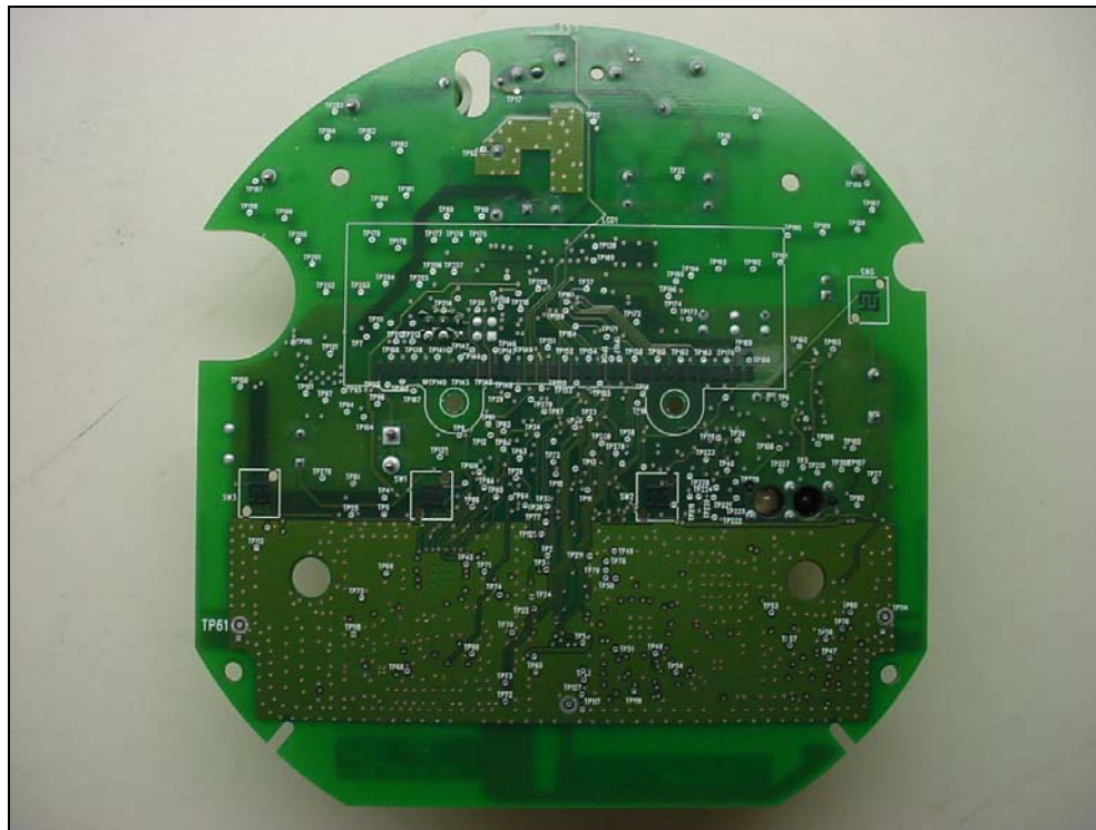
Figure 5: PCB - Back
