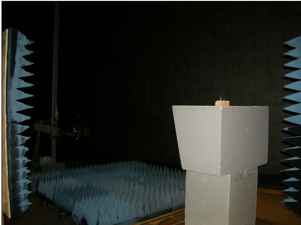
Figure 3: Radiated Emissions
