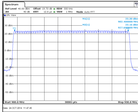
Figure 7.4.2.2-11: Mode 4 (64 Channels)
