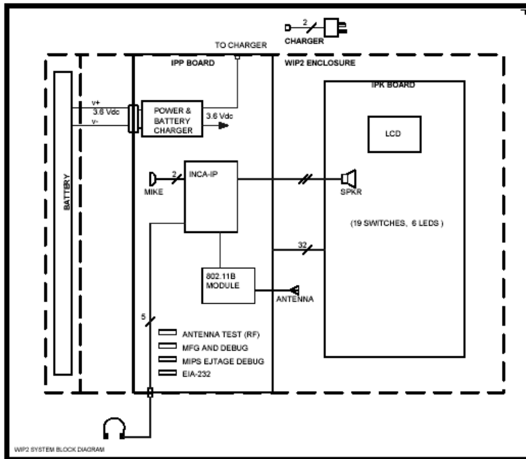
Figure 3: WIP2 System Block Diagram
