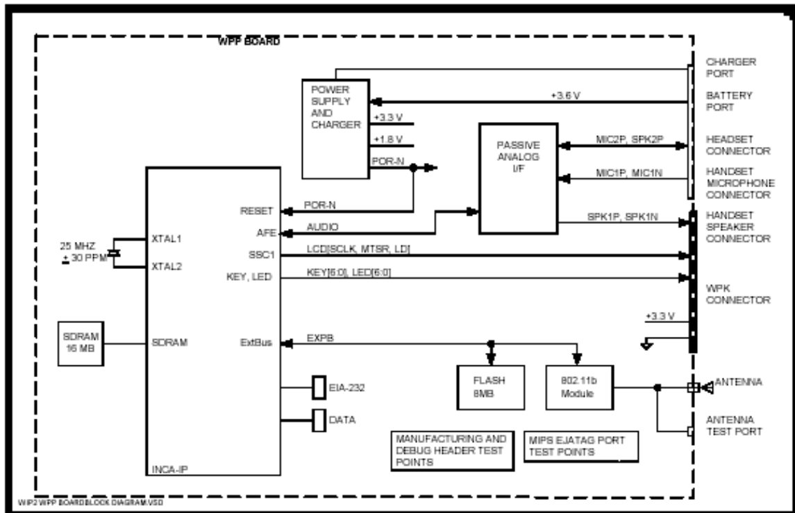
Figure 4: WPP Board Block Diagram
