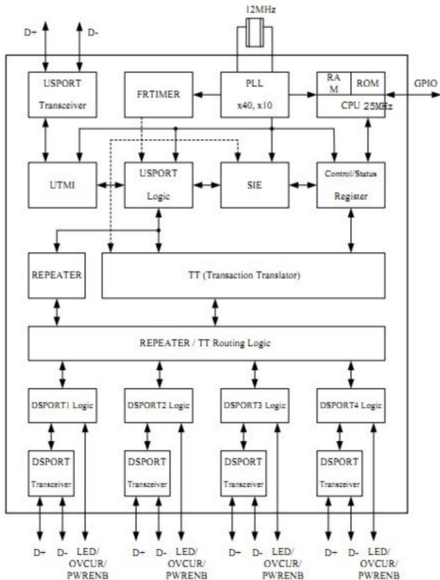
Figure 4.1 – GL850G Block Diagram (single TT)
