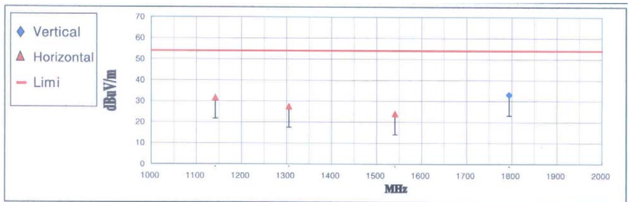
< Fig 7. Radiated Emission result _ Digital (1000MHz ~ 2000MHz) >
