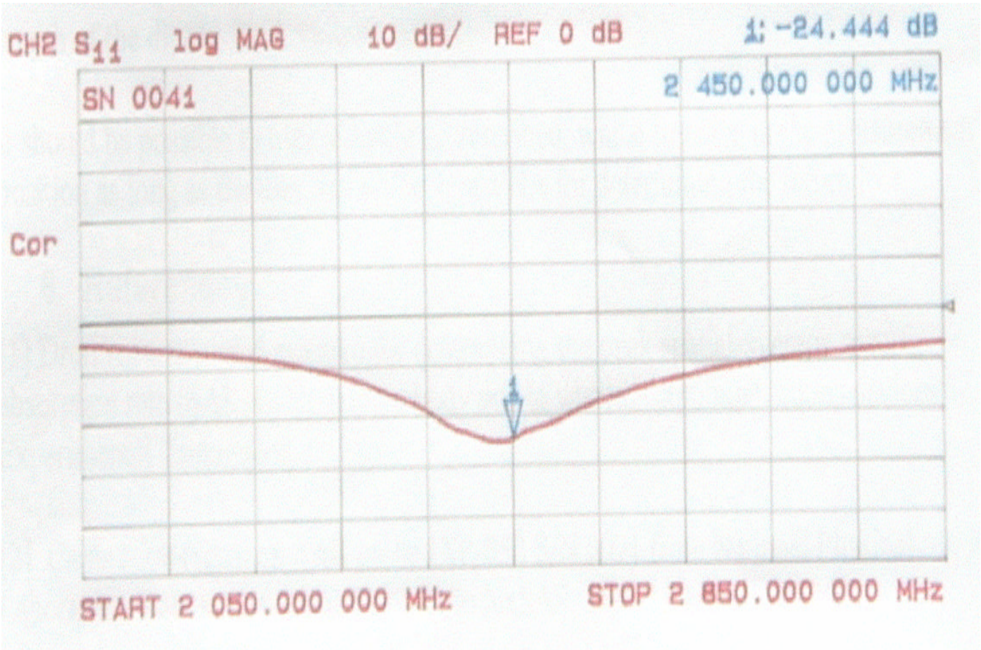
2450MHz dipole MFR return loss data.
