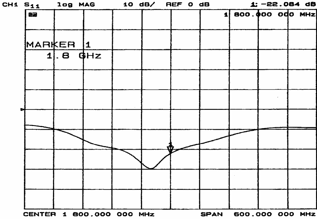
1800MHz Dipole MFR return loss Data
