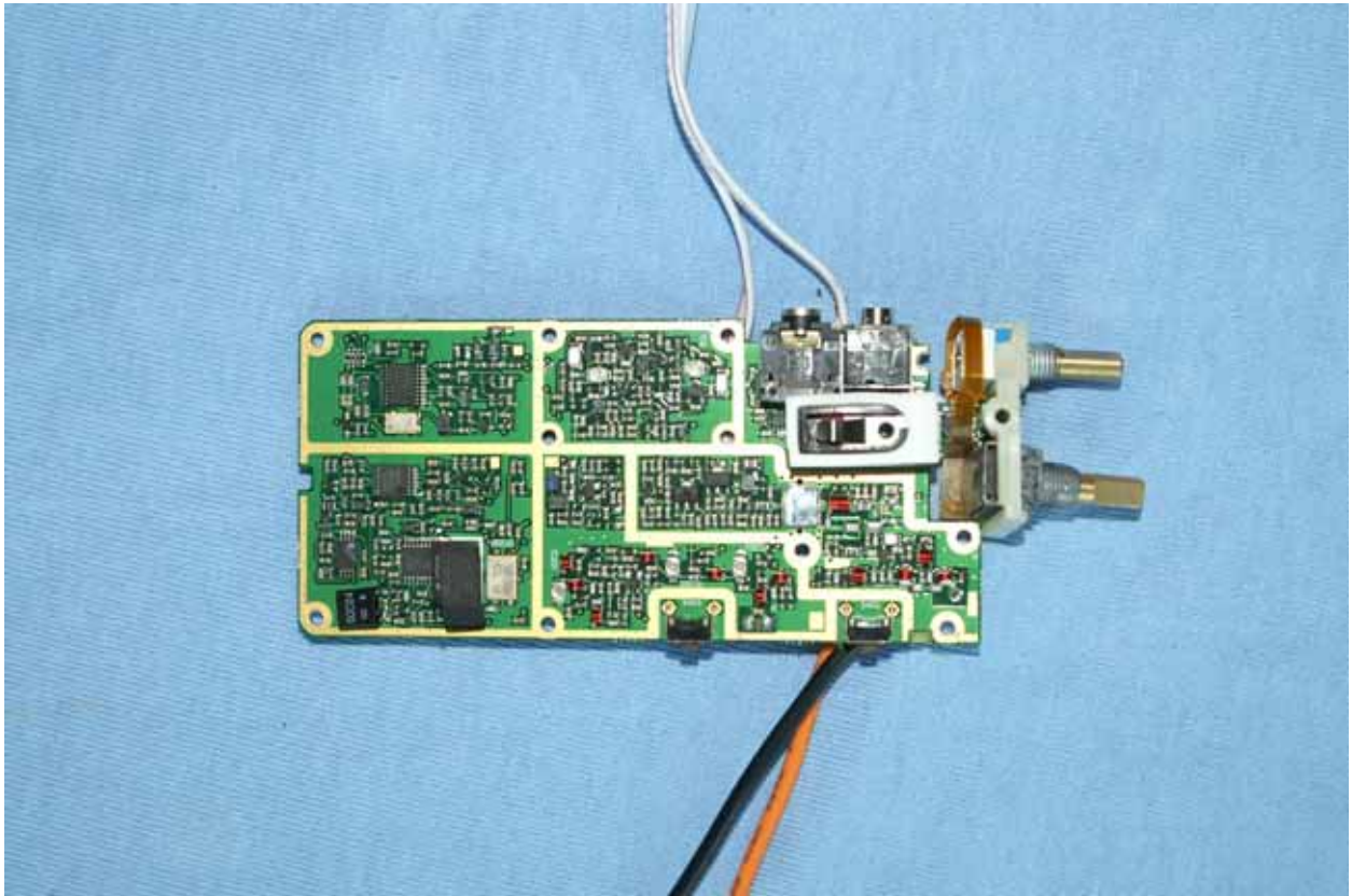
Detached view of EUT-9
