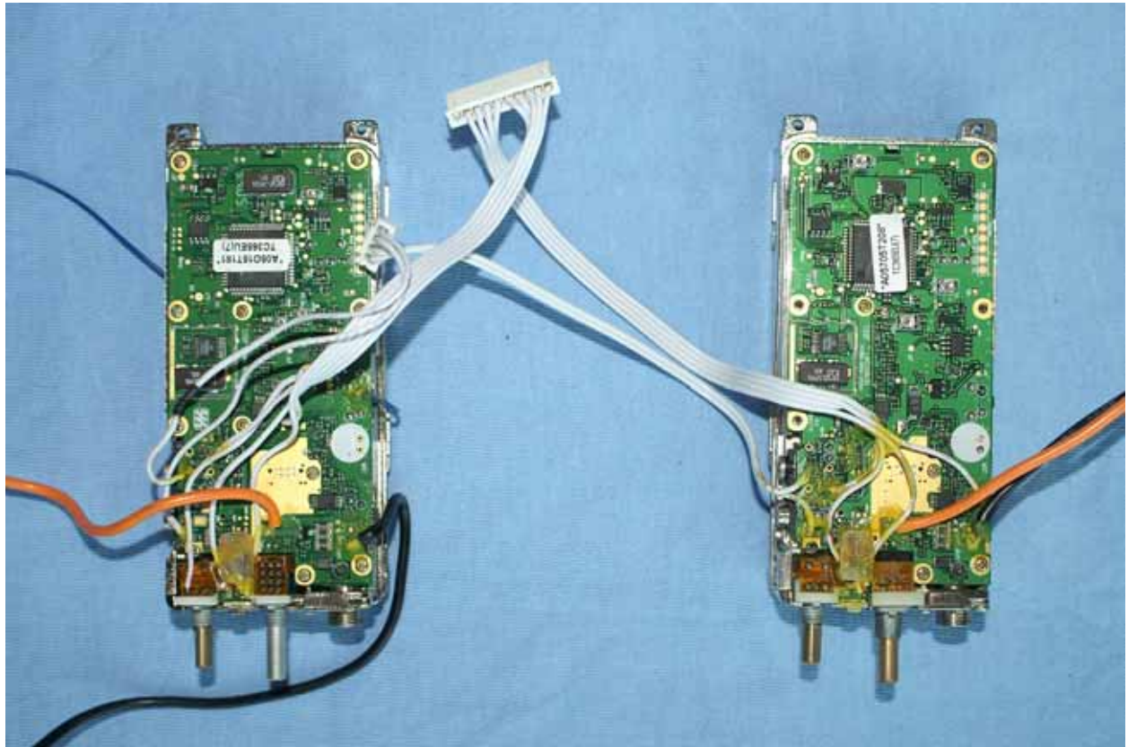
Detached view of EUT-7
