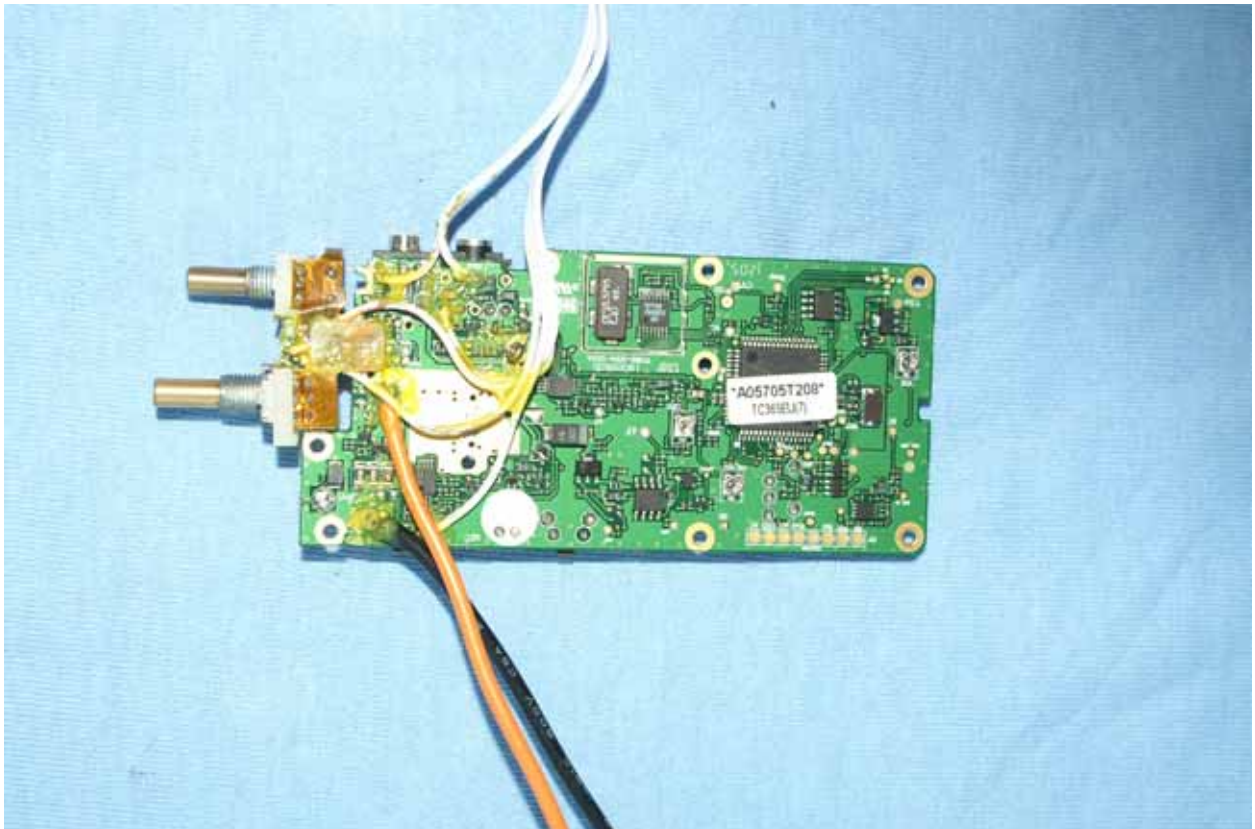
Detached view of EUT-10
