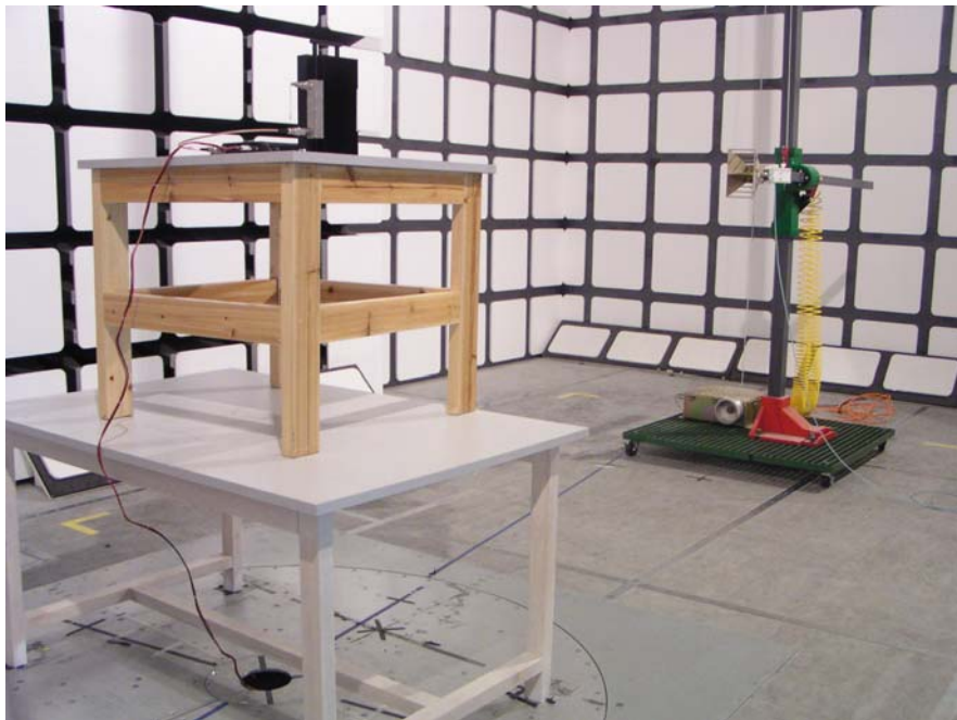
Radiated Emission - Rear View (Above 1000 MHz)
