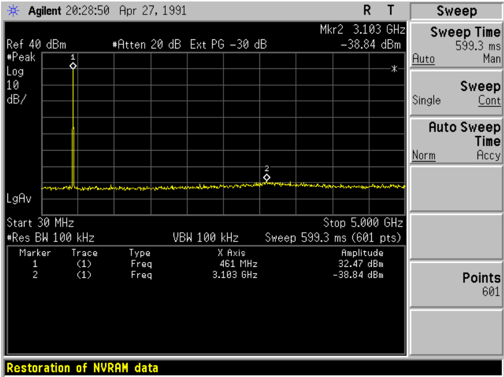
The Worst Case (5W@12.5KHz Channel space) of The Three Channels for Conduct Spurious Emission
