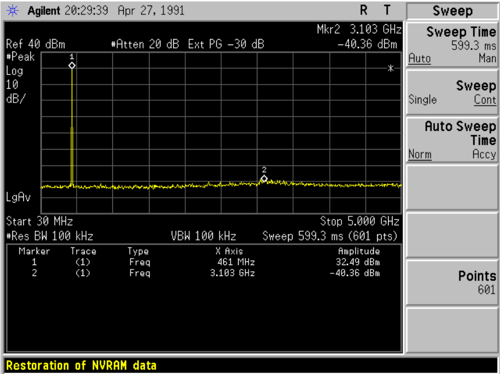
The Worst Case (5W@25.0 KHz Channel space) of The Three Channels for Conduct Spurious Emission
