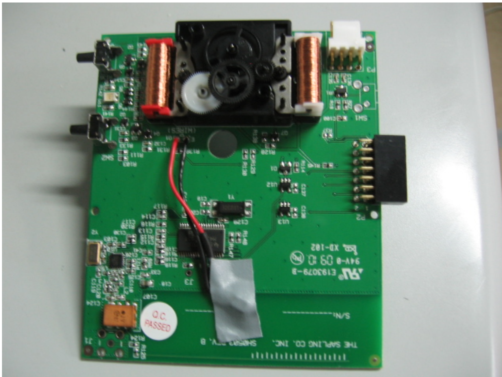
Figure 4: Clock Gears component open
