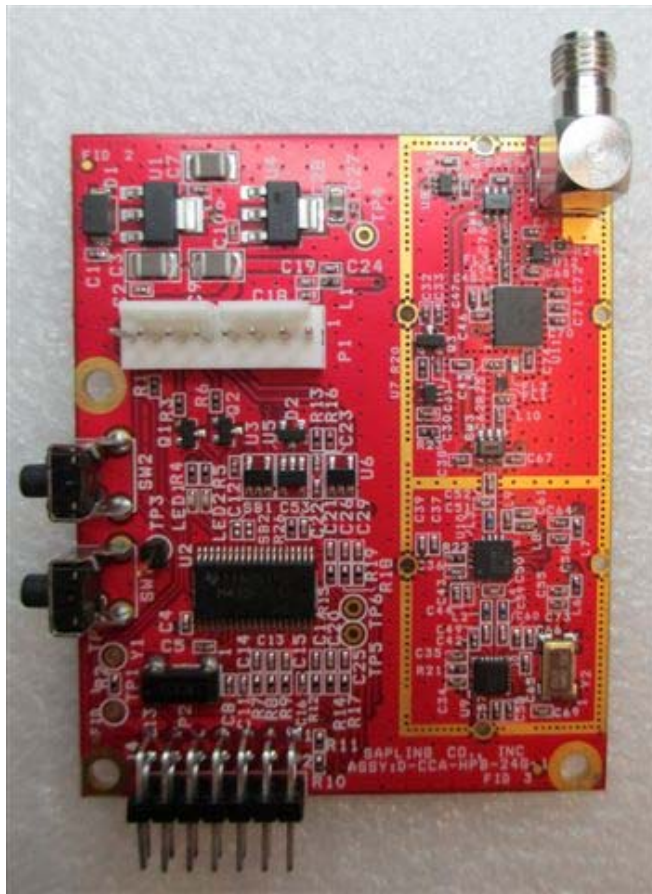
Model Number: D-CCA-HPB-24G-1, Internal Photograph, Top
