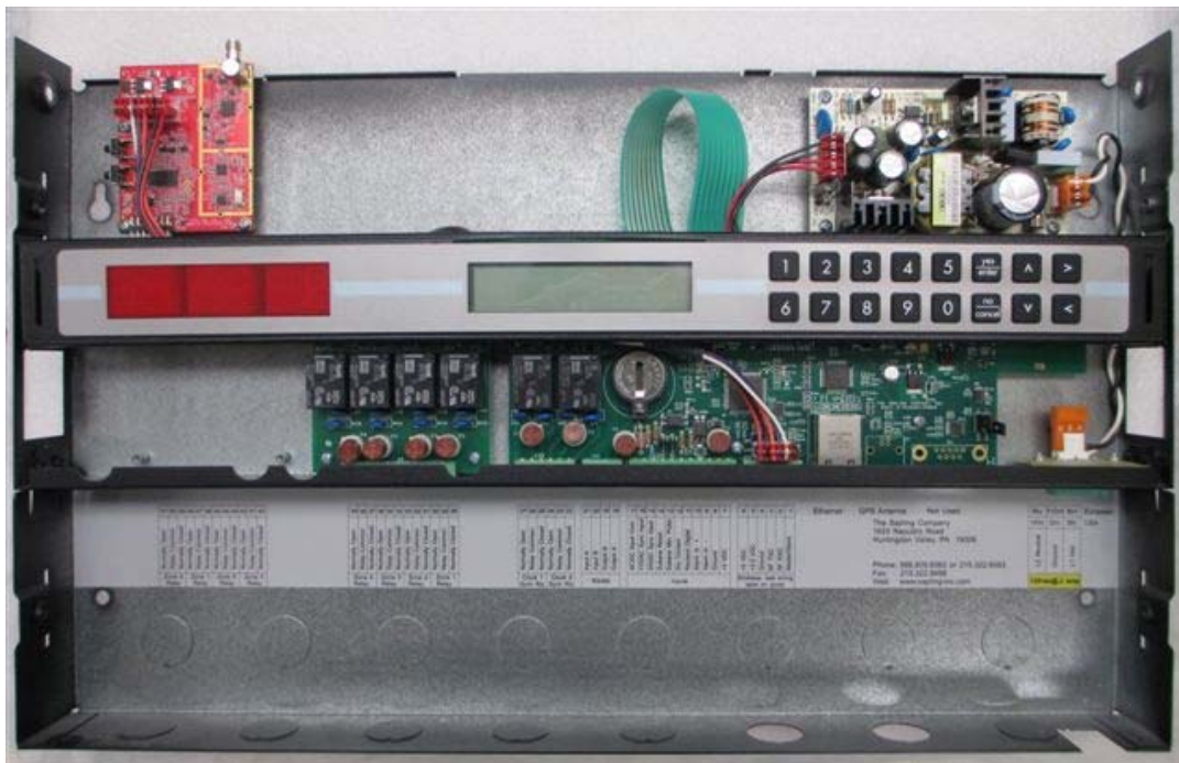
Model Number: D-CCA-HPB-24G-1 installed in SMA-3S0-G008-1 (Clock), Internal Photograph
