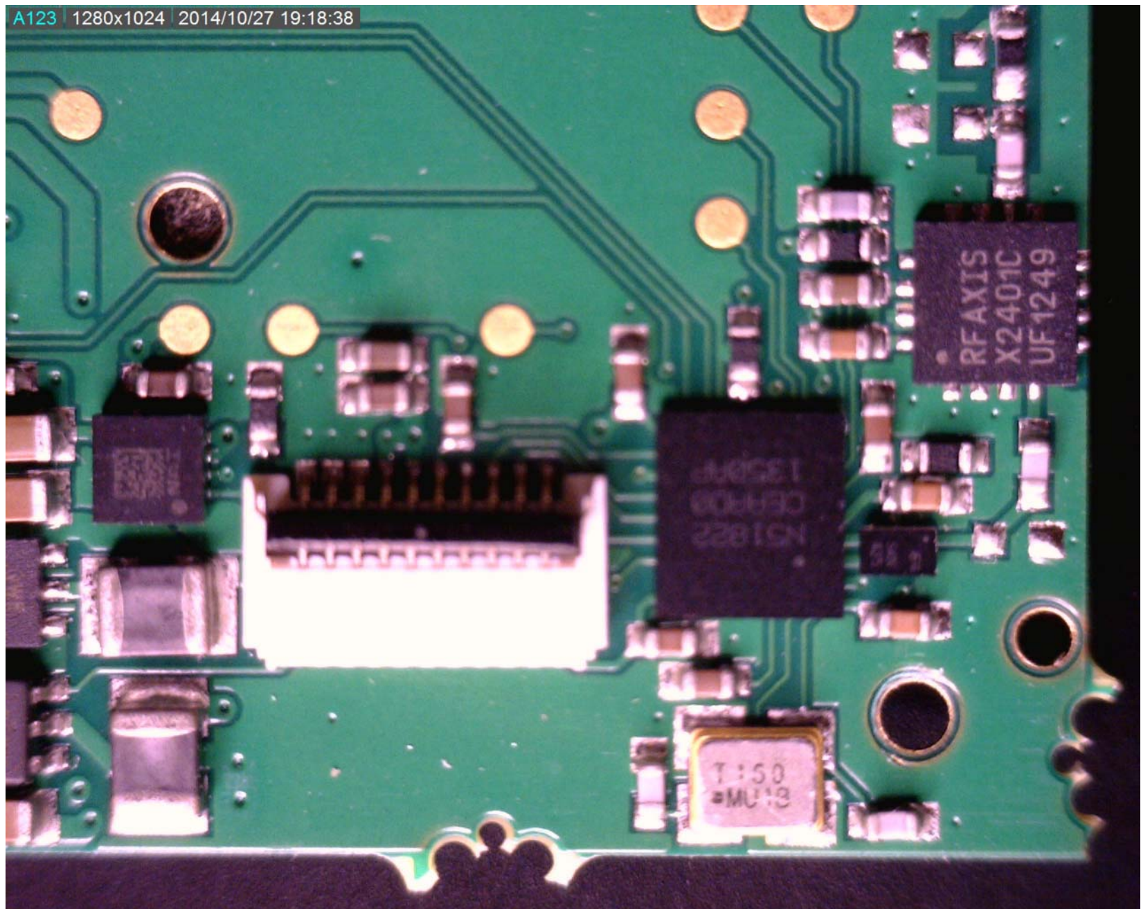
Figure 3 - Lively Watch - Radio Section of the PWB
