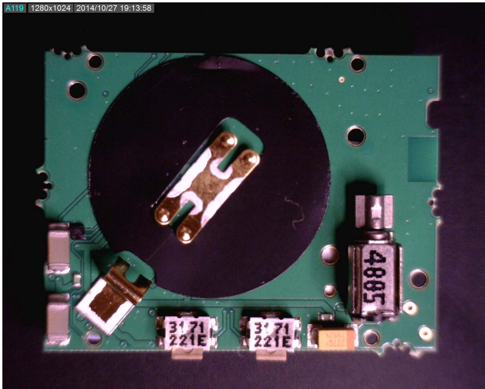
Figure 2 - Lively Watch - Back of the PWB
