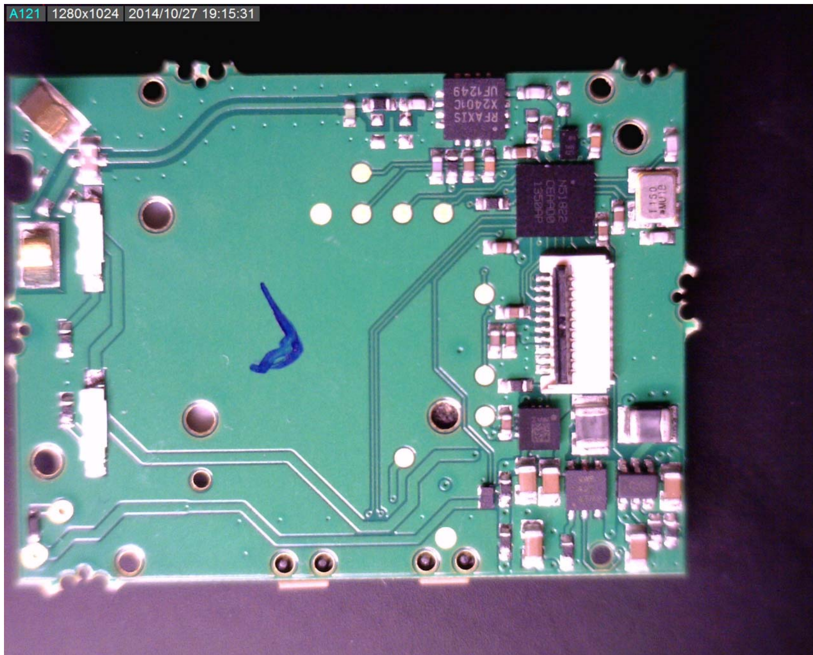
Figure 1 - Lively Watch - Front of the PWB
